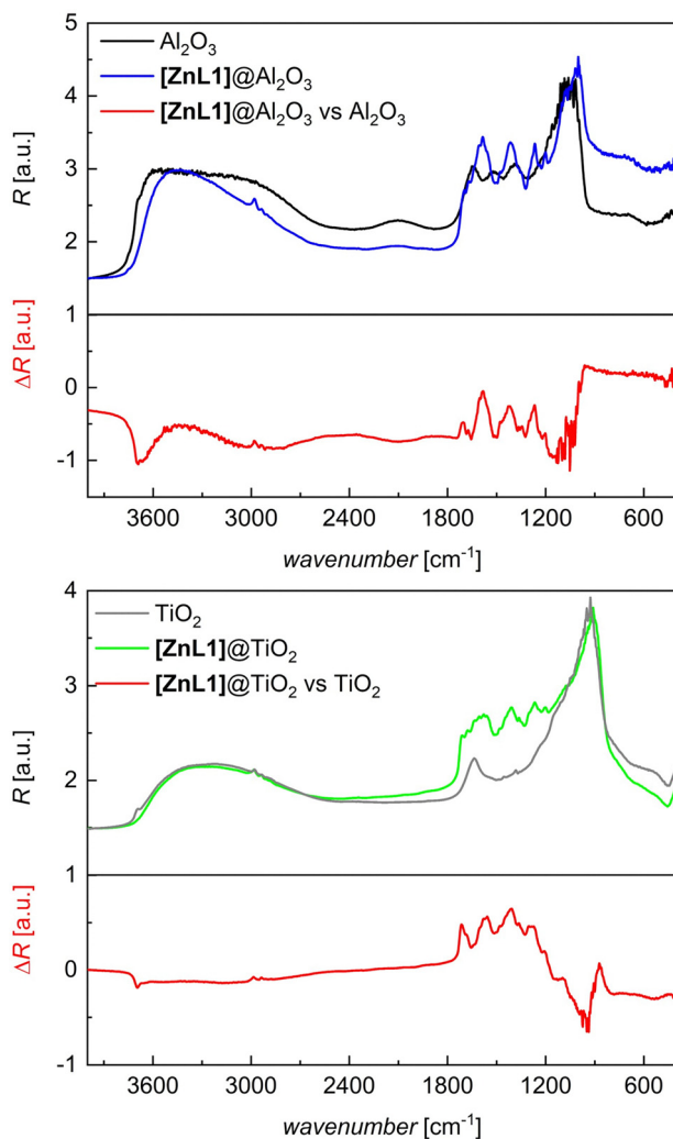
Fig. 2 DRIFT spectra of the substrates \text{TiO}_2 (grey) and \text{Al}_2\text{O}_3 (black), the immobilized complex [\text{ZnL1}] (blue, green) and the difference spectra (red).
