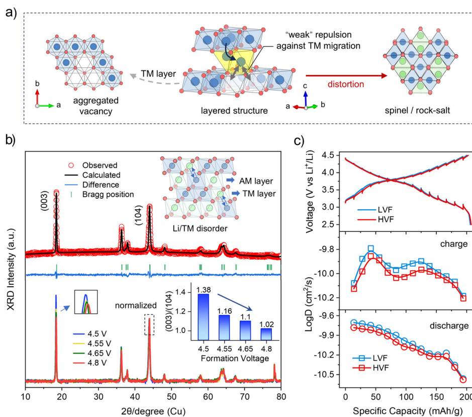
Figure 5. Stability of layered structure upon cycling. a) A schematic model illustrating phase changes from layered to spinel/rock salt. b) Ex situ XRD patterns and refined results of different formation voltages after 200 cycles. Insets present the peak intensity ratio of (003)/(104) and the enlarged view of the (003) crystal plane. c) GITT voltage curve and chemical diffusion coefficient [ \log(D_{Li^+}) ] of HVF and LVF cycling after 100 cycles.
