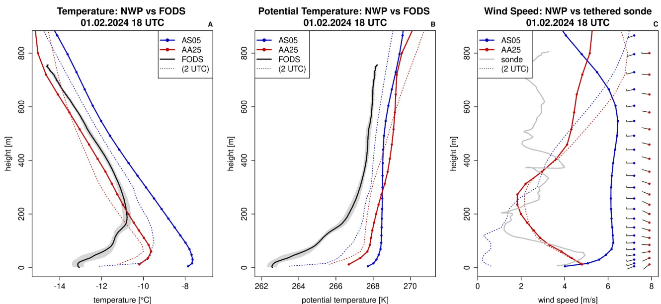
Figure 9. Same as Figure 7 on 01.02.2024 18 UTC. In addition, the dotted lines represent the respective (potential) temperature and wind speed profiles from AS05 and AA25 on 02.02.2024 2 UTC.
