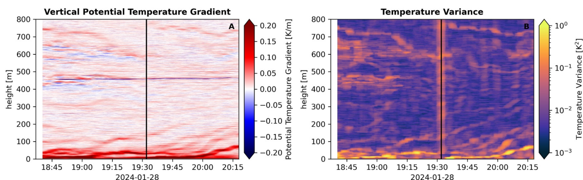
Figure 3. (a) Vertical potential temperature gradient and (b) temperature variance derived from fiber-optic distributed sensing (FODS) (with 5 min temporal average and 1 m spatial average) for flight 1 in Adventdalen on 28.01.2024. The vertical line in both panels marks the time when the FODS cold bath was stirred to resolve an unintended stratification.
