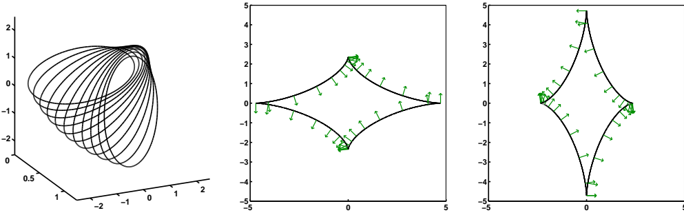
Figure 3: Funnel of F(\cdot) and derivative data \vec{DF}(0) and \vec{DF}(1)
