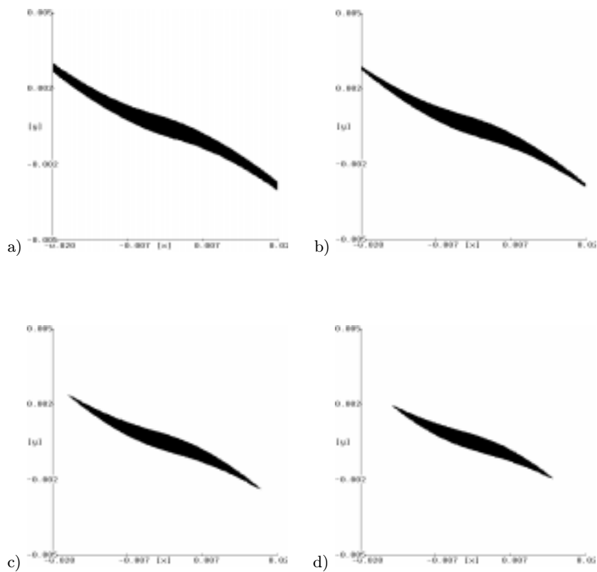
Fig. 2. Approximation of \mathcal{D}_0 for a) A = \{0\} , b) A = [-1, 1] , c) A = [-2, 2] , and d) A = [-3, 3]
