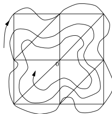
Fig. 1. A situation of non-convergence
