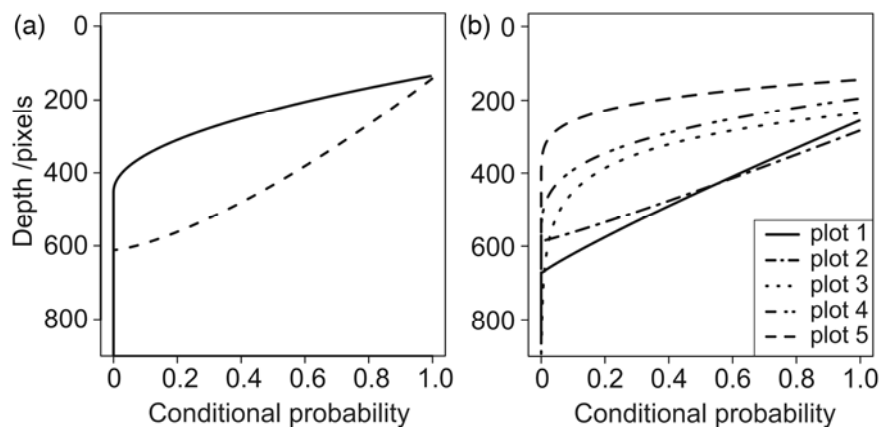
Figure 2.1.7 (a): Probability distribution for Brilliant Blue (solid line) and iodine–starch patterns (dashed line) on plot 4. (b): Probability distributions of the superposed Brilliant Blue stained profiles. The depth of the profiles is about 600 pixels, so in case of plots 1, 2 and 3 the dye reached the bottom of the profile.
