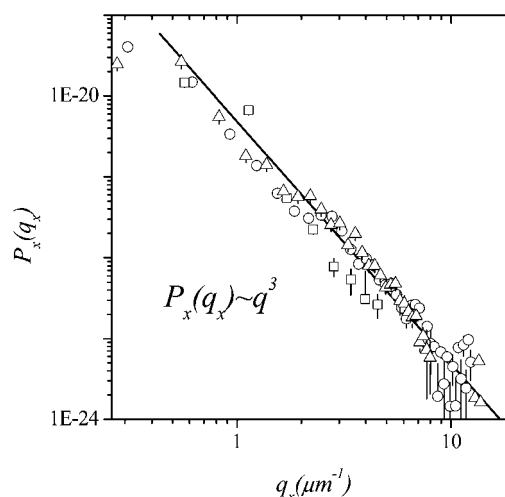
Fig. 7 Typical spectra of the shape fluctuations of giant L121-polymersomes. Data correspond to three different vesicles. The amplitudes follow a q_x^{-3} decay (straight line), characteristic of a pure bending motion. These fluctuations are well described by the Helfrich spectrum with a bending modulus, \kappa = 3 \pm 0.6 k_B T .
