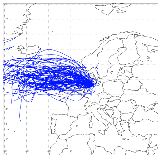
Cluster 4 (n=13)
