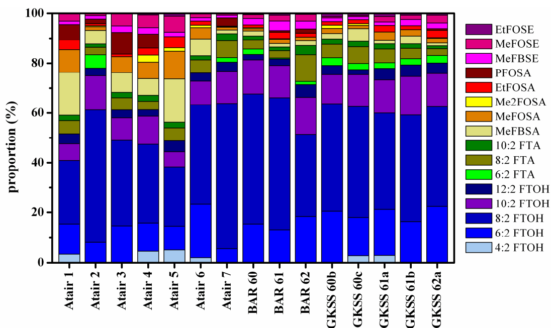
Figure 3-2: Proportions (%) of volatile PFC in gas-phase samples.
