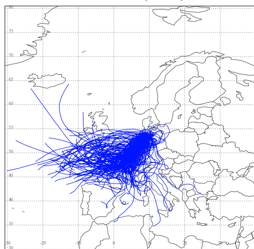
Cluster 6 (n=30)
