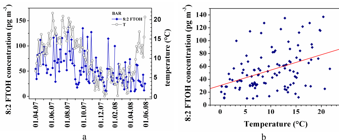
Figure 2-6: Local temperature (°C) and gas-phase concentrations (pg m -3 ) of 8:2 FTOH at Barsbüttel. a: Temperature and concentration course over the entire sampling period. b: Correlation of 8:2 FTOH and temperature. R=0.4. Note that high concentration events were excluded for these considerations.
