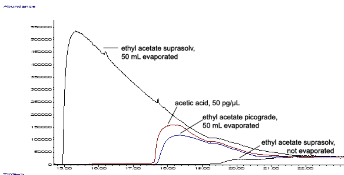
Figure 1-3: SIM chromatograms of acetic acid ( m/z 61, \text{CH}_3\text{CO}(\text{OH}_2)^+ ) in evaporated ethyl acetate SupraSolv, evaporated ethyl acetate Picograde, ethyl acetate SupraSolv that did not undergo evaporation, and an acetic acid standard solution ( 50 \text{ pg } \mu\text{L}^{-1} ) in ethyl acetate using a 30 m Supelcowax10 capillary column.
