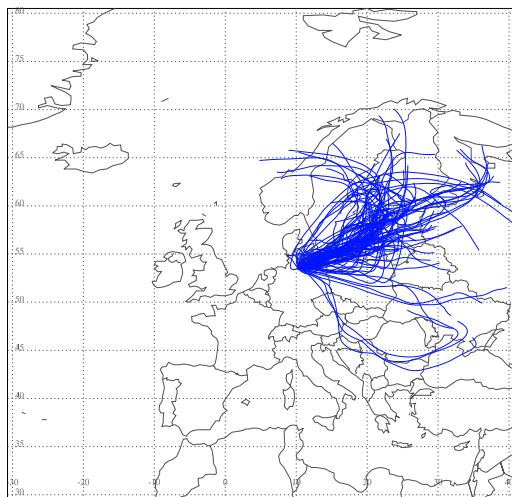
Cluster 1 (n=12)
