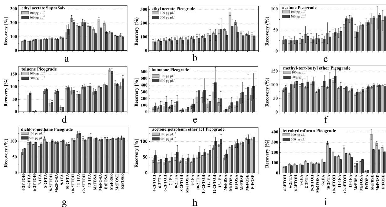
Figure 1-1: Average analyte recoveries ( n=3 ) of different solvents at concentrations of 100 \text{ pg } \mu\text{L}^{-1} and 500 \text{ pg } \mu\text{L}^{-1} . Error bars are standard deviations. The analytes were measured using a 30 m Supelcowax10 capillary column and are aligned according to their retention time. a: ethyl acetate SupraSolv, b: ethyl acetate Picograde, c: acetone, d: toluene, e: butanone, f: methyl tert-butyl ether, g: dichloromethane, h: acetone:petroleum ether 1:1 (v:v), i: tetrahydrofuran. Note the differences in the ordinates' scale.
