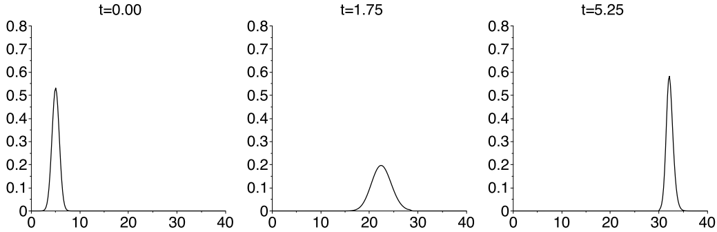
Fig. 1. Transport of the initial density into [30, 40] using MPC without density dependent speed constraint
