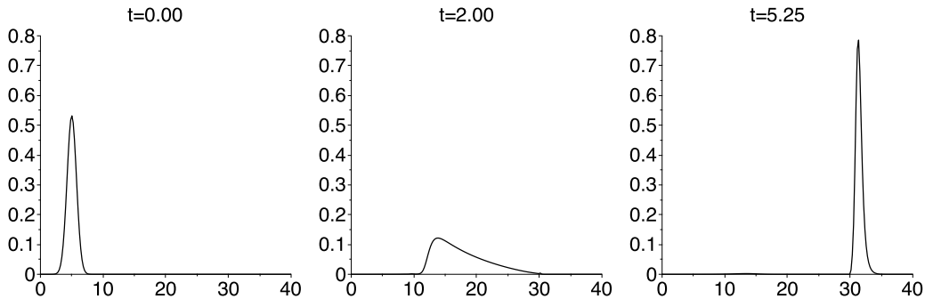
Fig. 2. Transport of the initial density into [30, 40] using MPC with density dependent speed constraint
