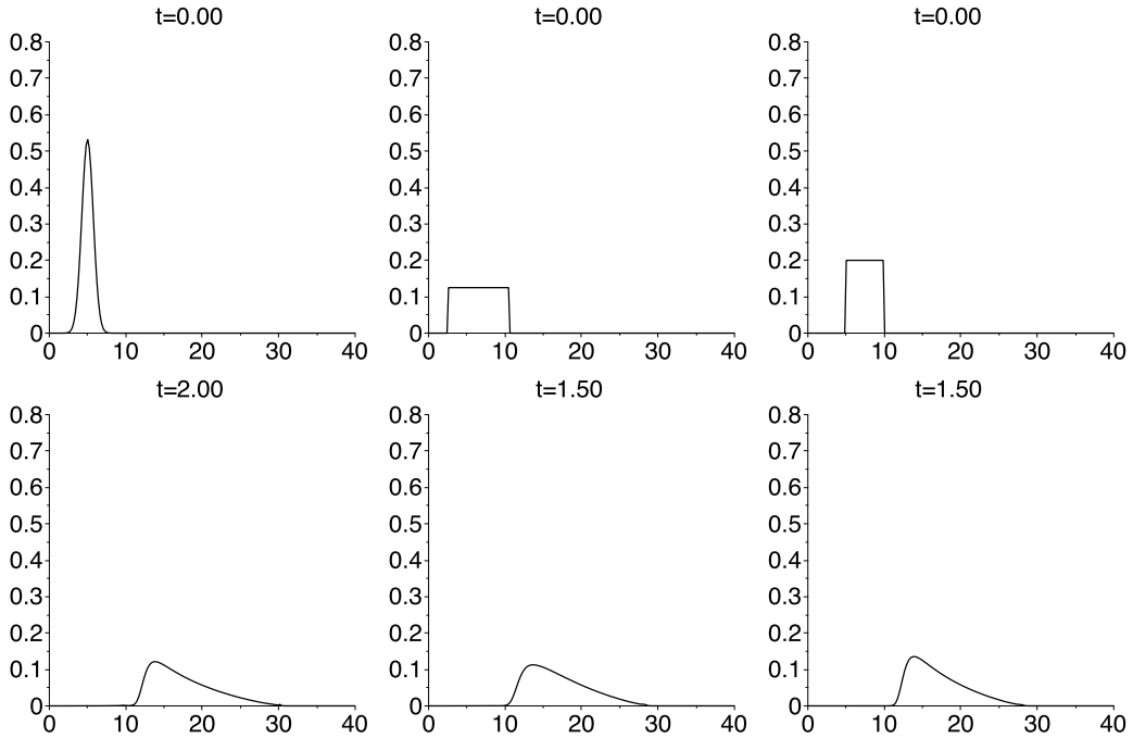
Fig. 4. Similarity of MPC solutions for different initial conditions (left to right) after a couple of time steps, indicating the occurrence of turnpike behavior
