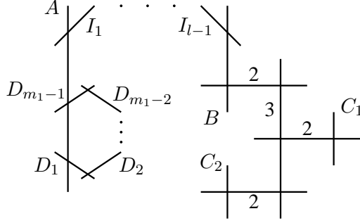
Figure 3.6: The special fiber of reduction type [I_{m_1} - IV^* - l]
