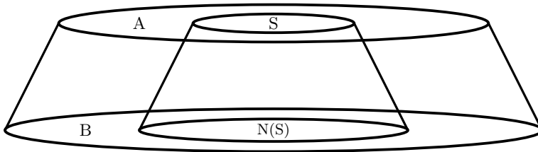
Fig. 1. A well-spread bipartite graph.
