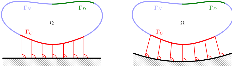
Fig. 1 Reference configurations of one body contact problems
