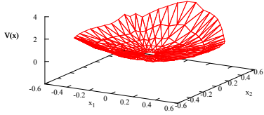
FIGURE 5.6. Numerical ISS Lyapunov function V(x) delivered by the algorithm for system (5.1), \epsilon = 0.048 , r = 0.420909 .
