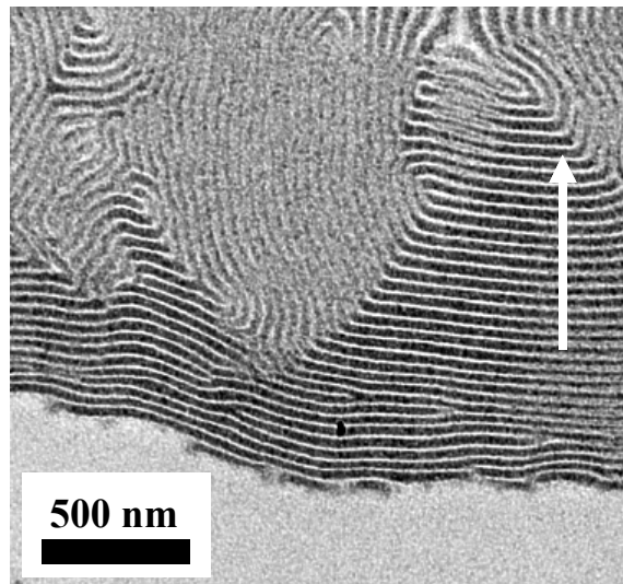
Figure 5-6: TEM picture of interfacial region between electric field aligned polymer film and electrode surface (Film embedded in epoxy resin. The arrow indicates the direction of the electric field vector).
