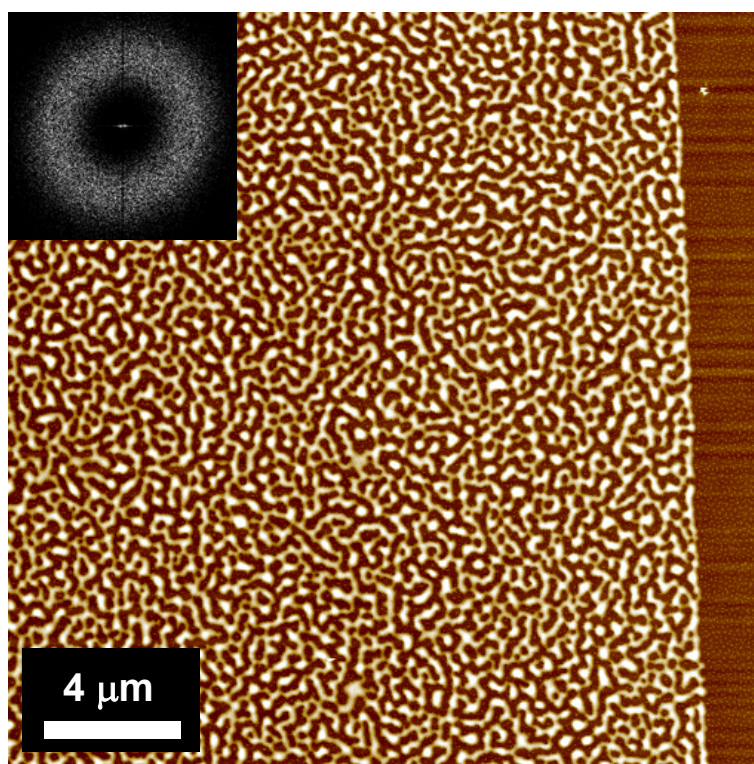
Figure 4-3: SFM topography image of PS 54 on S_{48}2VP_5M_{47}^{180} after 5 min at 130 °C (z-range: 60 nm). Fourier-transform of the PS pattern (inset) yields d \sim 420 nm.
