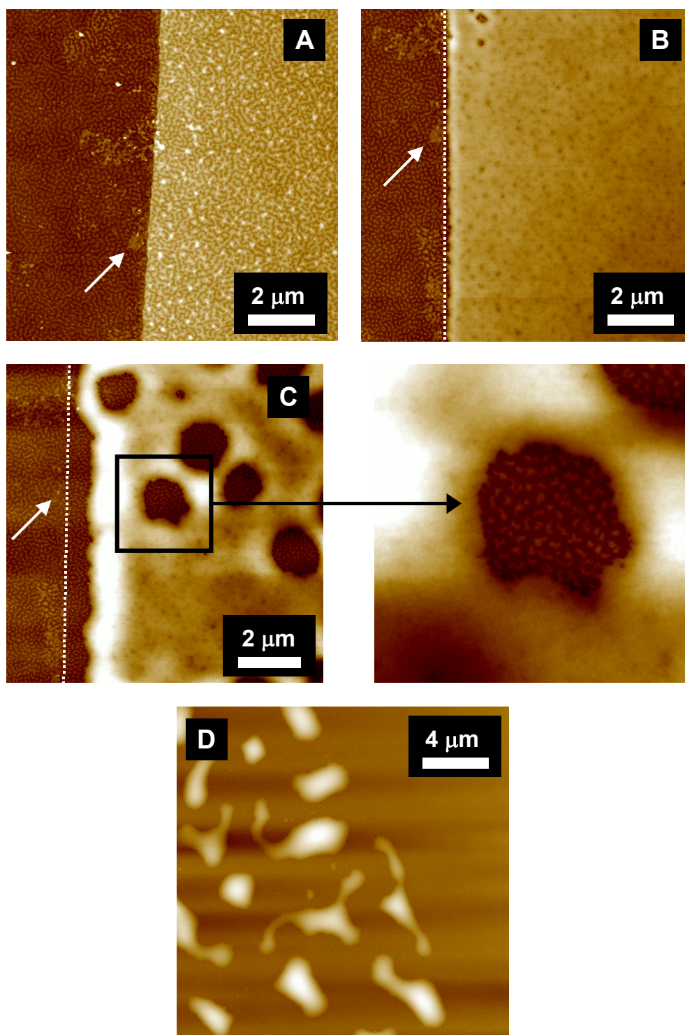
Figure 4-5: SFM topography images of PS 104 on S_{48}2VP_5M_{47}^{180} (A) as prepared, (B) after 3 min (C) 9.5 min ( z -range: 50 nm) and (D) 15 min saturated CHCl_3 vapor ( z -range: 250 nm). The dotted lines show the original position of the rim. The arrow points to a defect in the sublayer.
