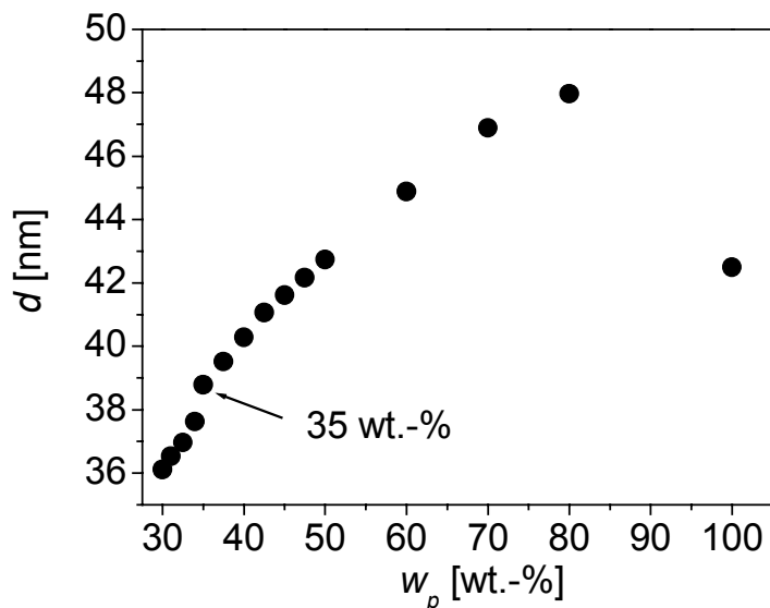
Figure 6-3: Concentration dependence of the lamellar spacing of PS-b-PI solutions in toluene ( d_{\text{bulk}} = 42.5 nm).
