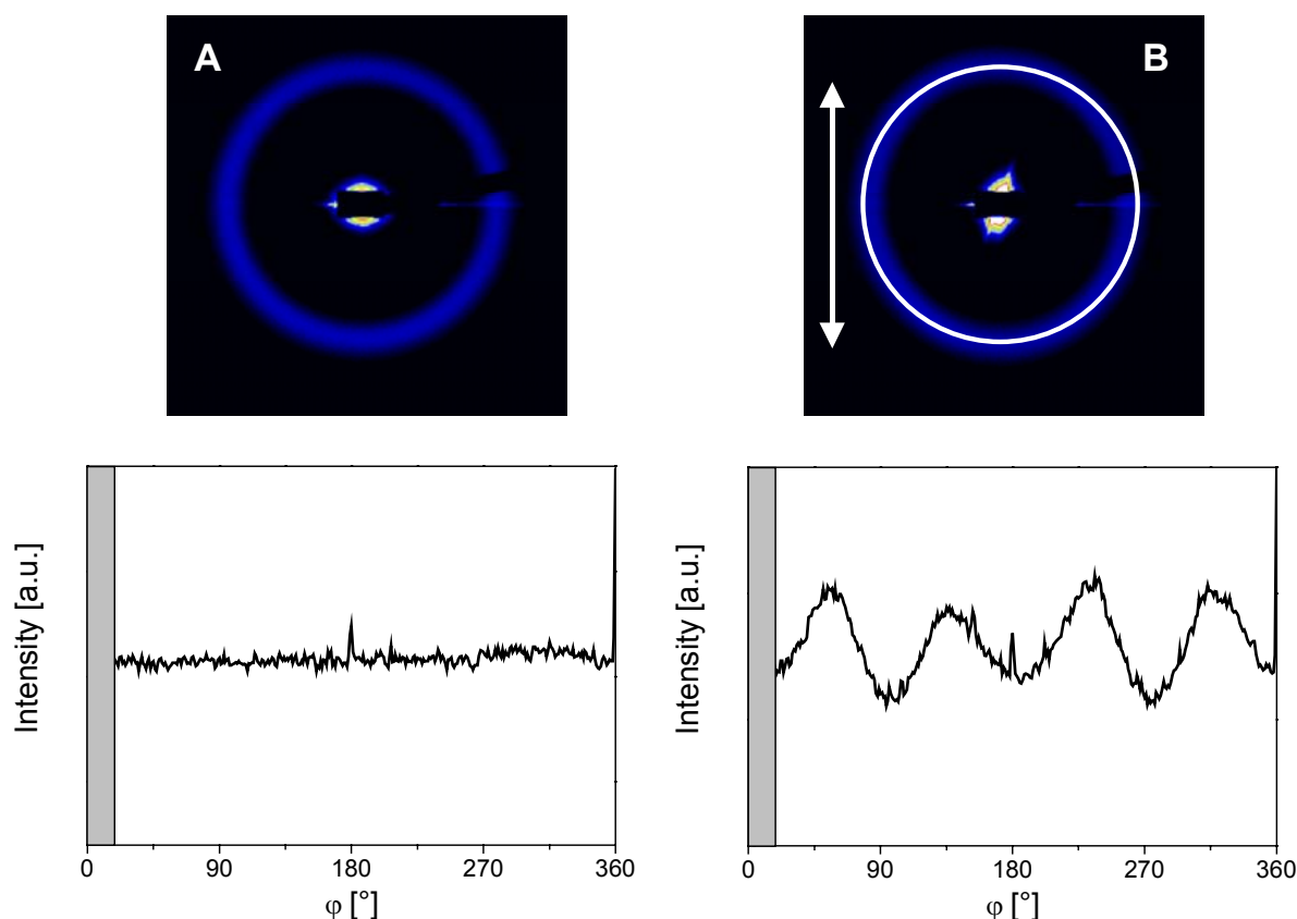
Figure 7-8: 2D SAXS patterns and respective azimuthal angular dependence of scattering intensity of a 50 wt.-% solution of S_{49}M_{51}^{100} in THF. (A) Before and (B) after application of an electric field of strength E = 5 \text{ kV/mm} .
