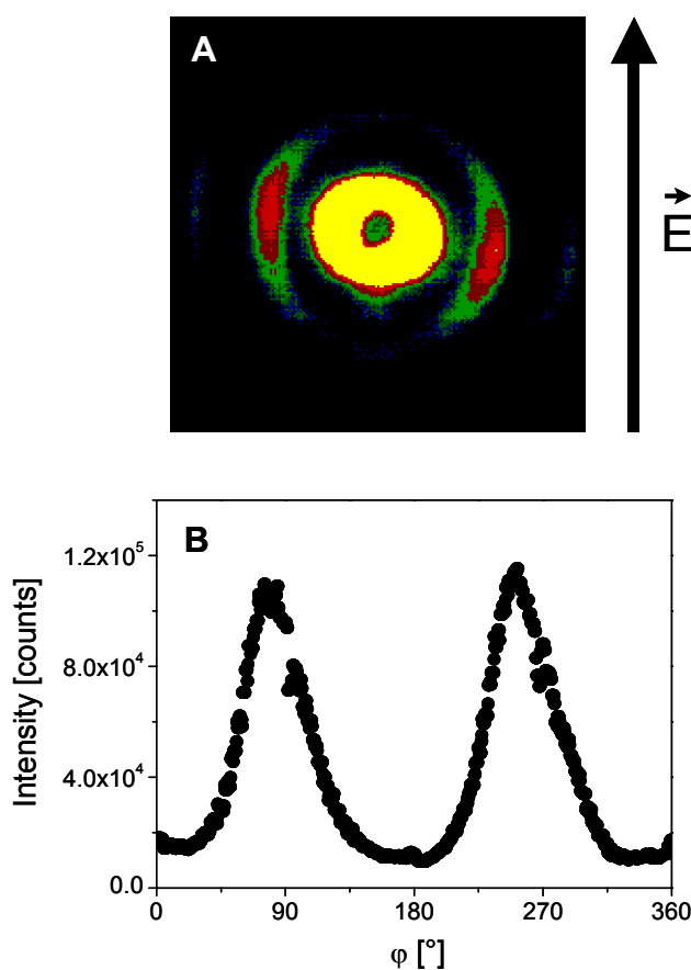
Figure 5-8: (A) SAXS pattern of a sample taken from the flat areas in between the columns. The lamellae are oriented along the field direction (1.8 kV/mm), however the degree of order as calculated by the azimuthal angular dependence of the scattering intensity (B) is smaller than within the columns ( P_2 = -0.25 compared to -0.4 ).
