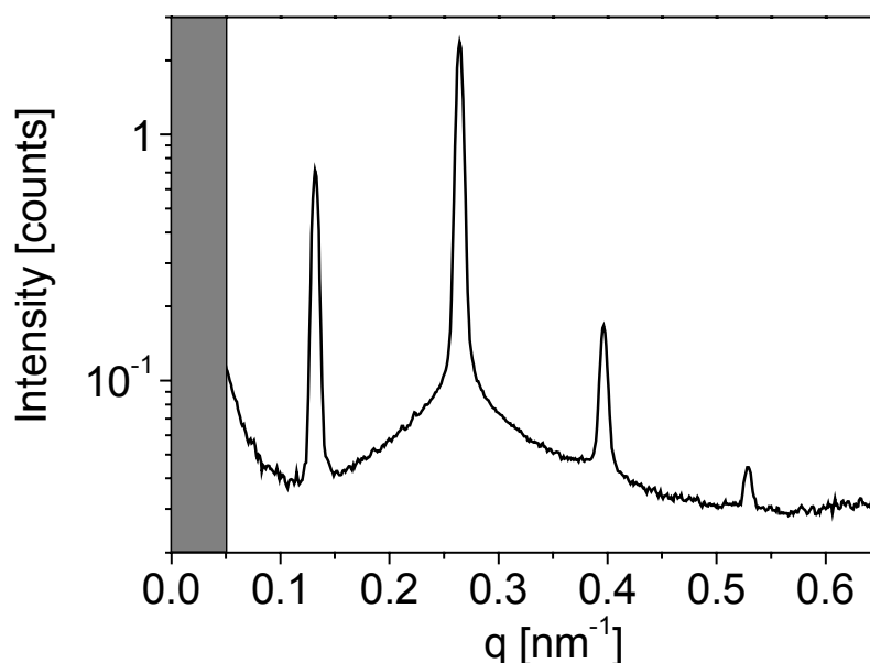
Figure 8-9: Scattering intensity profile of a 40 wt.-% solution of S_{27}V_{35}T_{38} 84 in THF.
