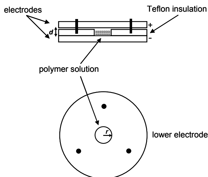
Figure 5-1: Capacitor setup used for sample preparation in the absence and in the presence of an electric field, respectively.
