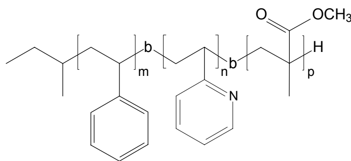
Figure 4-1: Chemical structure of PS- b -P2VP- b -PMMA triblock copolymer ( N_{PS} = 825 , N_{P2VP} = 80 , N_{PMMA} = 855 ).
