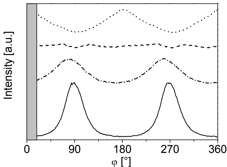
Figure 8-4: Azimuthal angular dependence of the scattering intensity for a 40 wt.-% S_{50}V_{50}^{78} solution in THF exposed to an electric field of E = 1 kV/mm: 0 sec (.....), 5.6 sec (---), 16.4 sec (---), 50.6 sec (—).
