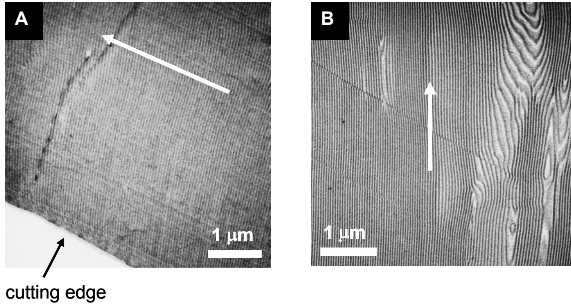
Figure 5-3: TEM pictures of zero-field and alignment experiment. (A) zero-field (The arrow indicates the direction perpendicular to the electrodes). (B) E = 1.8 \text{ kV/mm} (The arrow indicates the direction of the electric field vector). The image was taken from one of the columns bridging between the electrodes.
