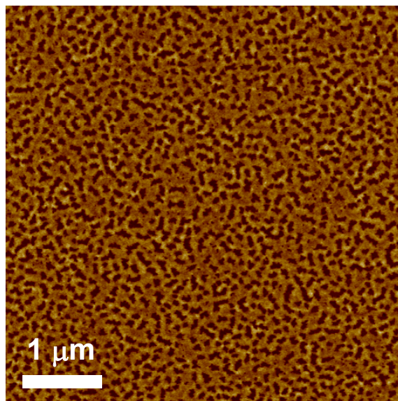
Figure 3-7: SFM micrograph of ultrathin film of S_{48} 2VP_5 M_{47}^{180} dip-coated from 0.1 mg/ml THF solution onto a polished silicon wafer. Z-range: 8 nm.
