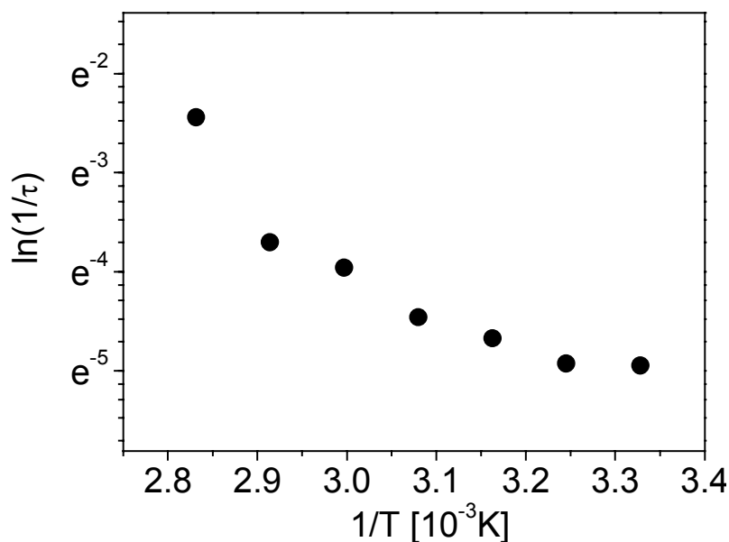
Figure 6-12: Arrhenius plot for the temperature dependence of the rate constant, 1/\tau , for a 47.5 wt.-% solution in toluene.
