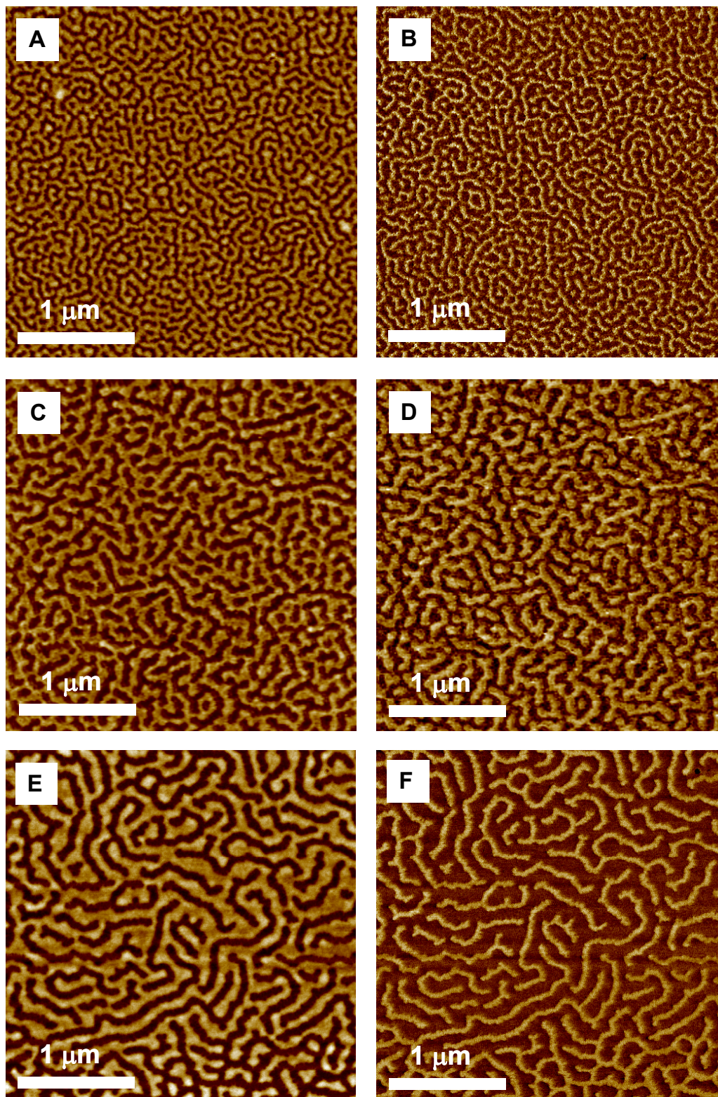
Figure 3-3: SFM micrographs and phase images of ultrathin films of PS- b -PHEMA- b -PMMA adsorbed from 1 mg/ml THF solutions onto a polished silicon wafer. (a, b) S_{47}H_{10}M_{43}^{82} ; (c, d) S_{46}H_4M_{50}^{134} ; (e, f) S_{67}H_6M_{27}^{129} . Topography: 8 nm, Phase: 15 °.
