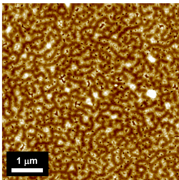
Figure 4-4: SFM topography image of PS 14 on S_{48}2VP_5M_{47}^{180} after 1 min of exposure to saturated CHCl_3 vapor (z-range: 15 nm).
