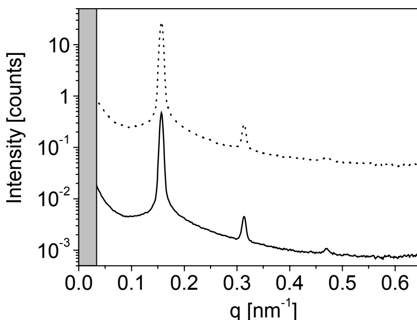
Figure 6-14: Scattering intensity profiles of a 37.5 wt.-% solution prior (····) and during (—) application of an electric field of E = 1 \text{ kV/mm} .
