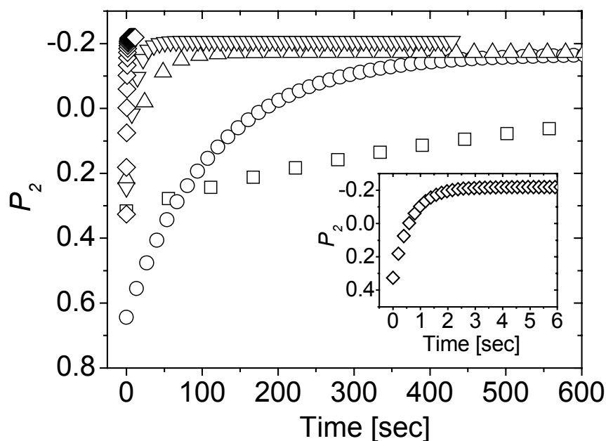
Figure 7-6: Evolution of orientational order parameter P_2 with time for 40 wt.-% solutions at different field strengths ( \square = 375 V/mm, \tau = 545 sec; \circ = 500 V/mm, \tau = 116 sec; \triangle = 1 kV/mm, \tau = 18.7 sec; \nabla = 1.5 kV/mm, \tau = 10.3 sec; \diamond = 3 kV/mm, \tau = 0.64 sec). Electrode spacing: 2 mm.
