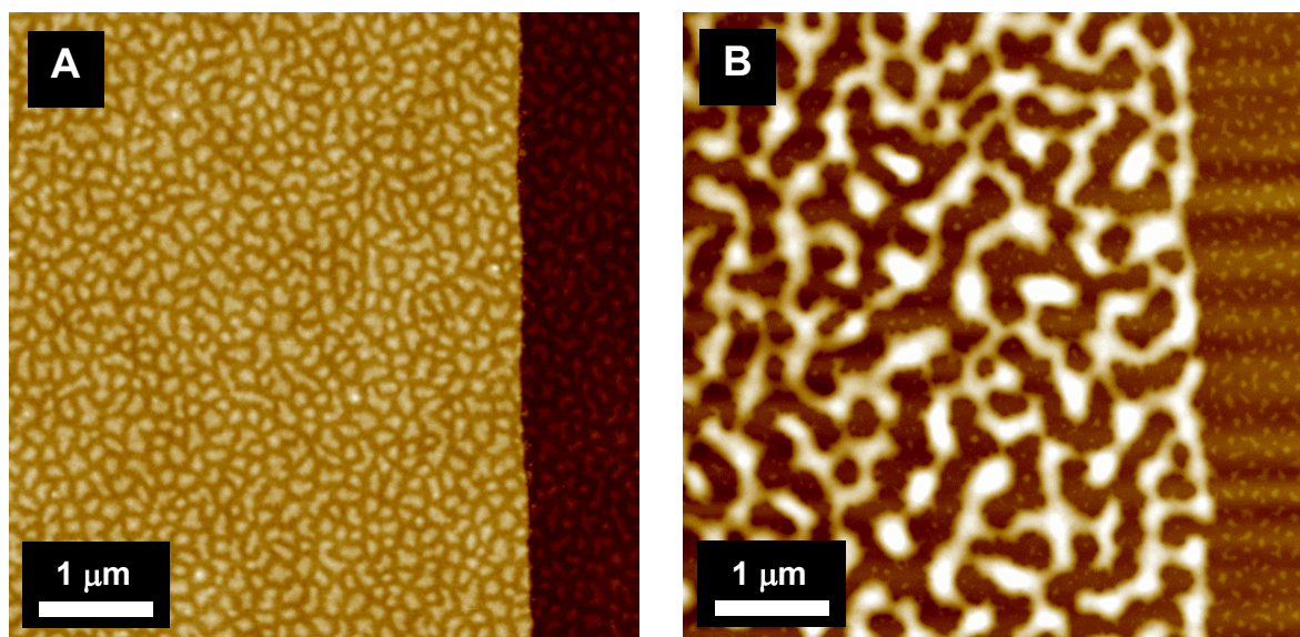
Figure 4-2: SFM topography image of PS 54 on S_{48}2VP_5M_{47}^{180} : (A) as prepared (z-range: 30 nm) and (B) after 5 min at 130 °C (z-range: 60 nm). The right side of each image shows the pure triblock copolymer substrate.
