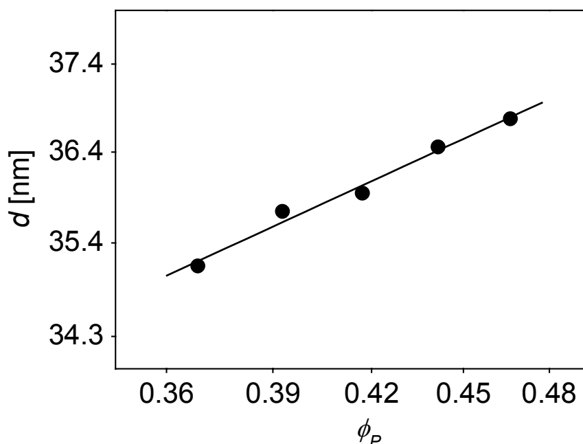
Figure 8-3: Double logarithmic plot of dependence of lamellar spacing on the volume fraction of polymer \phi_P for intermediate concentrations of S_{50}V_{50}^{78} in THF ( d \sim \phi_P^{0.21 \pm 0.02} ).
