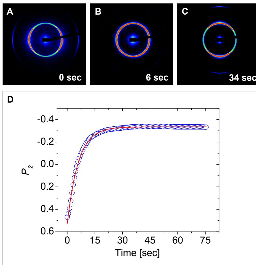
Figure 6-5: (A-C) Two-dimensional SAXS patterns of a 35 wt.-% solution of the SI-80 diblock copolymer in toluene taken at room temperature prior (A) and after application of an electric field ( E = 1 \text{ kV/mm} ) (B, C). (D) Time dependence of the orientational order parameter P_2 . The solid line is a least squares fit to the data according to Equation 6-3 with P_{2,0} = 0.52 , P_{2,\infty} = -0.32 , and \tau = 5 \text{ sec} .
