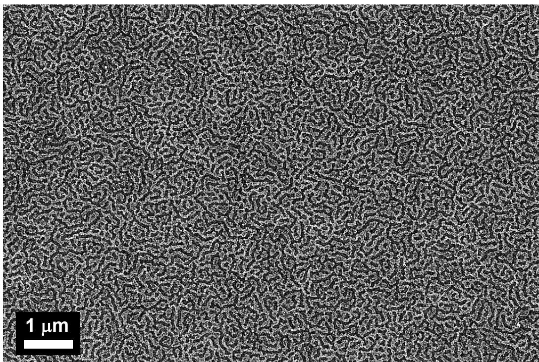
Figure 3-5: Large area SEM micrograph of an ultrathin film of S_{48} 2VP_5 M_{47}^{180} adsorbed from 1 mg/ml THF solution onto a polished silicon wafer
