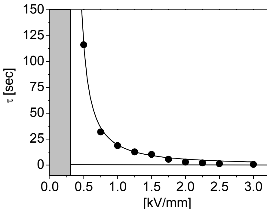
Figure 7-7: Electric Field dependence of time constant \tau for 40 wt.-% solutions. The solid line represents a least squares fit of the power law \tau = \alpha(E - E_t)^a + \tau_\infty to the data points yielding \alpha = 0.10 \text{ sec} , a = -1.47 , E_t = 310 \text{ V/mm} and \tau_\infty = 0 \text{ sec} .
