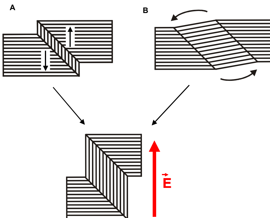
Figure 6-13: Schematic representation of proposed mechanisms: (A) migration of grain boundaries, (B) rotation of grains.
