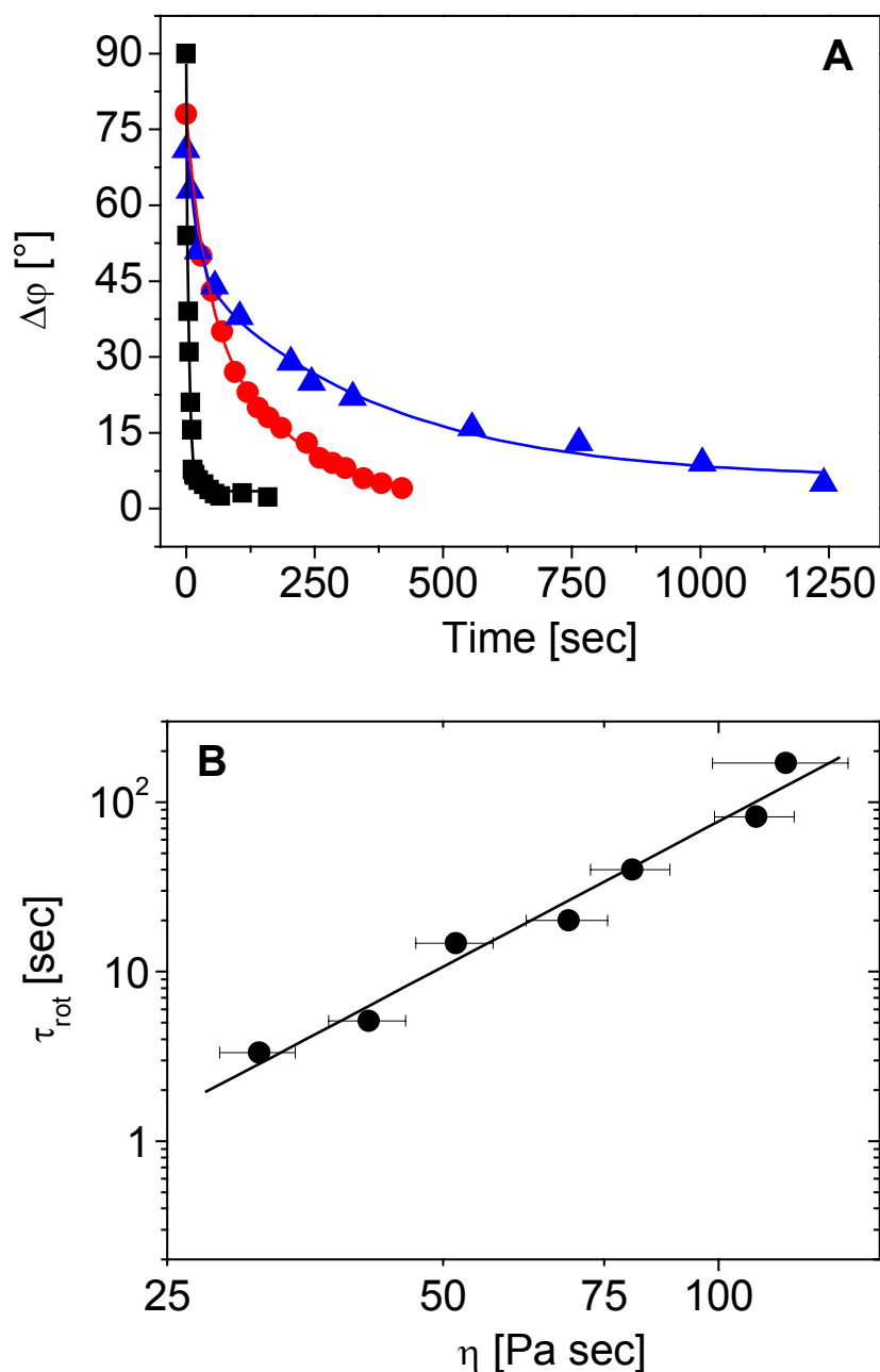
Figure 6-16: (A) Angular shift of rotational component at different concentrations (■ = 35 wt.-%, ● = 47.5 wt.-%, ▲ = 50 wt.-%) at field strength of E = 1 kV/mm at T = 25^\circ\text{C} . The solid lines represent the least squares fits to the data yielding the rotational time constant, \tau_{rot} ; (B) Double logarithmic plot of \tau_{rot} versus solution viscosity, \eta ( \tau_{rot} \propto \eta^{2.85 \pm 0.22} ).
