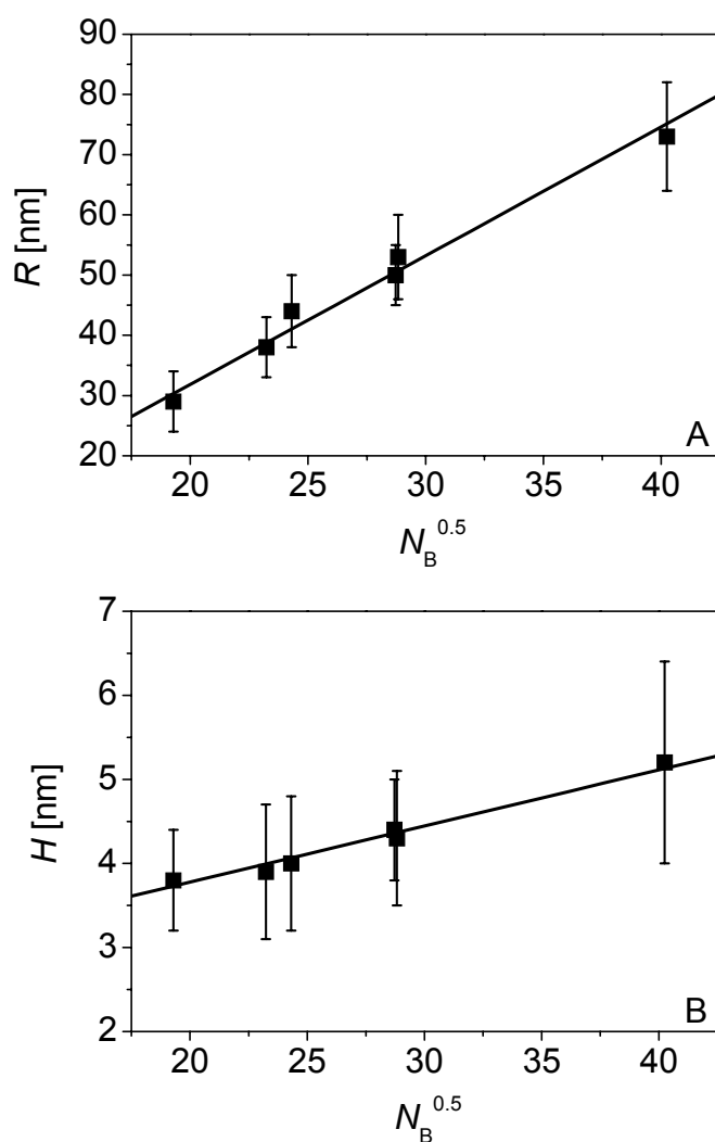
Figure 3-11: Scaling of PS- b -PHEMA- b -PMMA and PS- b -P2VP- b -PMMA stripe morphology according to Gaussian behaviour: (A) half-width R , (B) height H of PS stripes.
