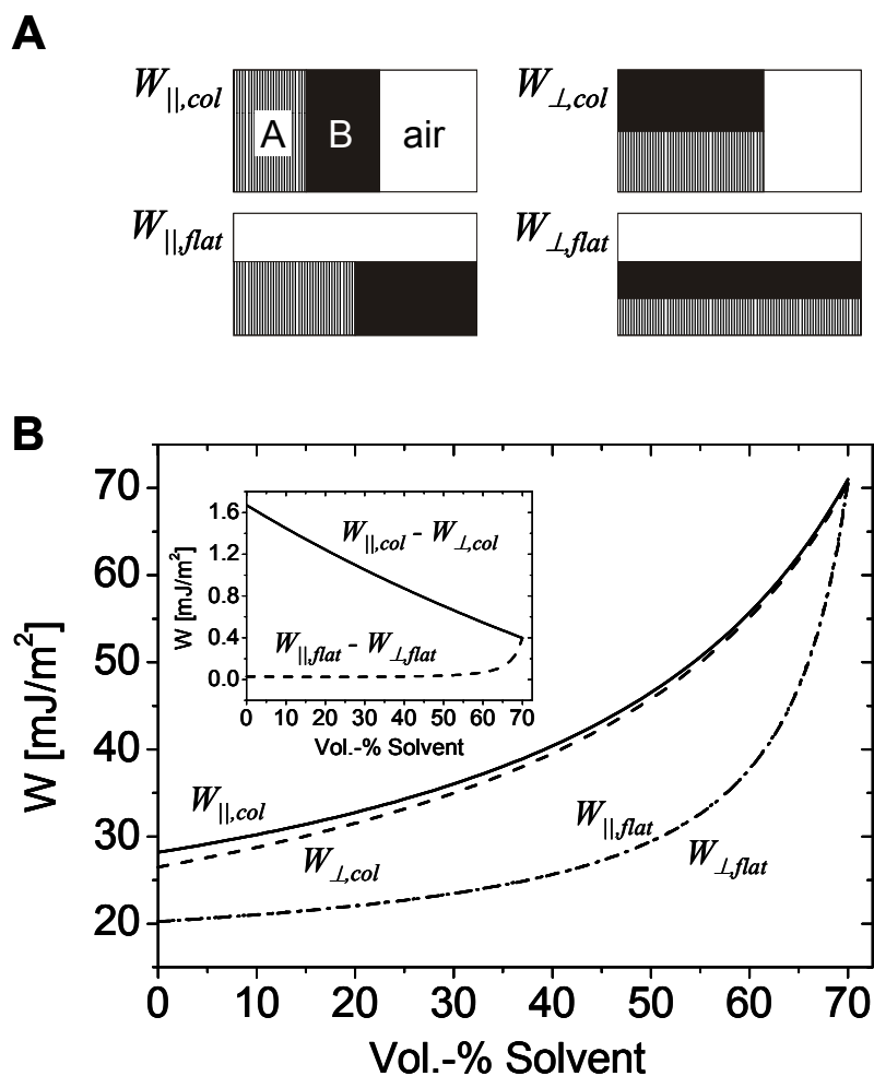
Figure 5-7: (A) Different geometries used for the calculation of the electric energy W stored in a capacitor partially filled with polymers A and B. (B) Energy per area stored in the capacitor for the four geometries as a function of solvent concentration. The inset shows the energy difference between the two orientations for columns ( W_{\parallel,col} - W_{\perp,col} ) and for a flat film ( W_{\parallel,flat} - W_{\perp,flat} ), respectively.
