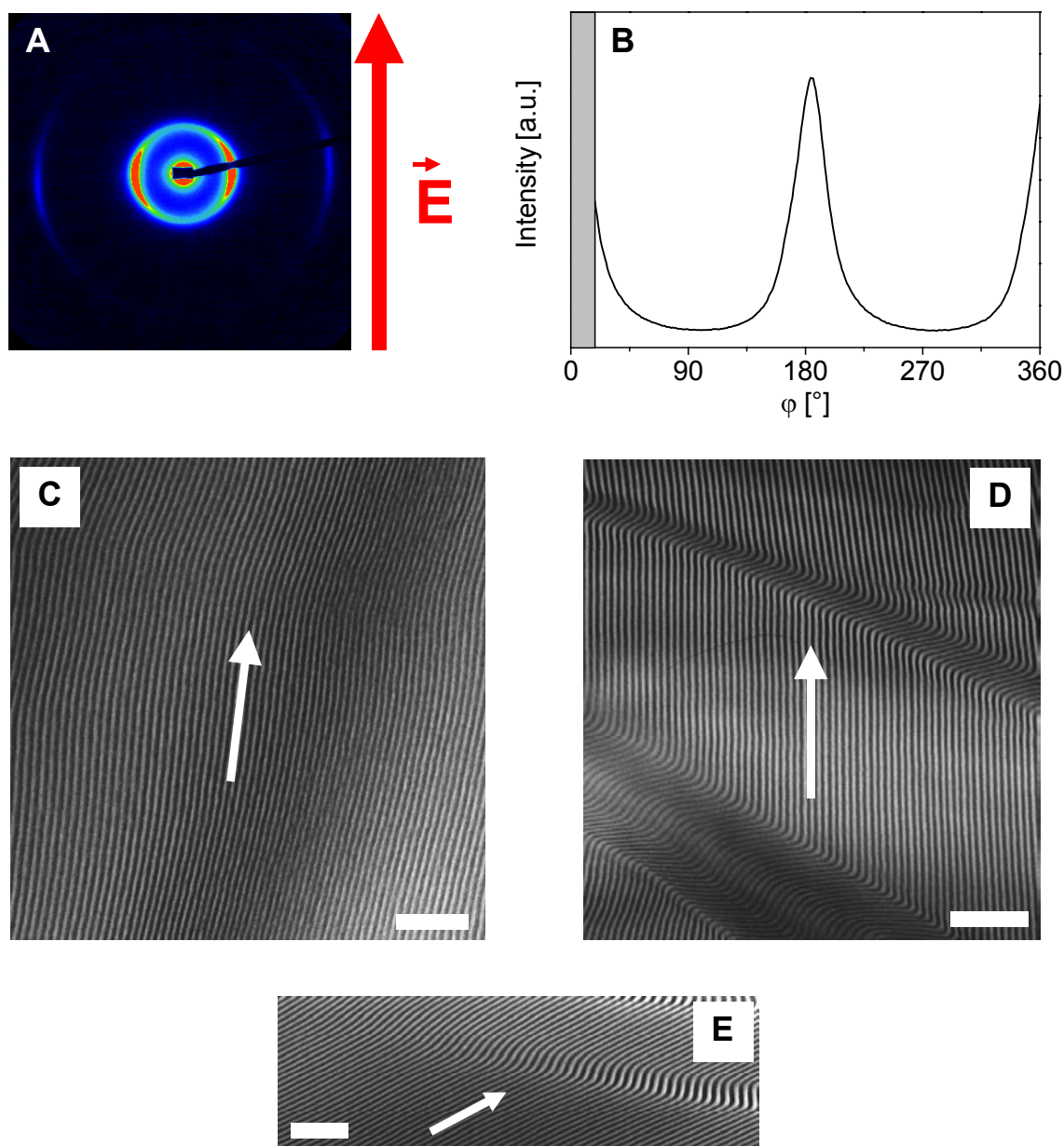
Figure 6-15: SAXS and TEM data of a bulk sample prepared from a 40 wt.-% solution of SI-80 in toluene dried under an applied electric field of 1 kV/mm. The arrows indicate the direction of the electric field vector. (A) 2D-SAXS pattern and (B) azimuthal intensity distribution at first order reflection ( P_2 = -0.34 ). The TEM pictures show a defect free domain (C) and characteristic kink band defects (D/E). The scale bar represents 400 nm.
