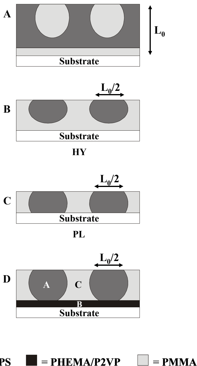
Scheme 3-4: Schematic depiction of proposed surface perpendicular morphologies for AB and ABC block copolymers.
