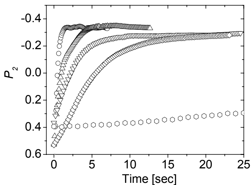
Figure 6-9: Evolution of orientational order parameter P_2 with time for 35 wt.-% solutions at different field strengths ( \circ = 375 \text{ V/mm} , \diamond = 1 \text{ kV/mm} , \nabla = 1.25 \text{ kV/mm} , \triangle = 1.5 \text{ kV/mm} , \circ = 3 \text{ kV/mm} , electrode spacing: 2 mm).
