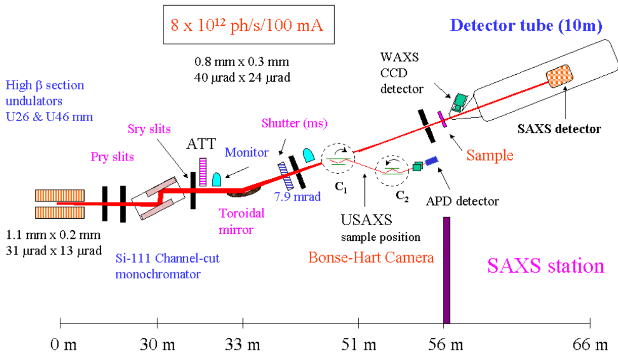
Figure 2-10: Setup of ID02A High-Brilliance Beamline at the ESRF, Grenoble (France)
