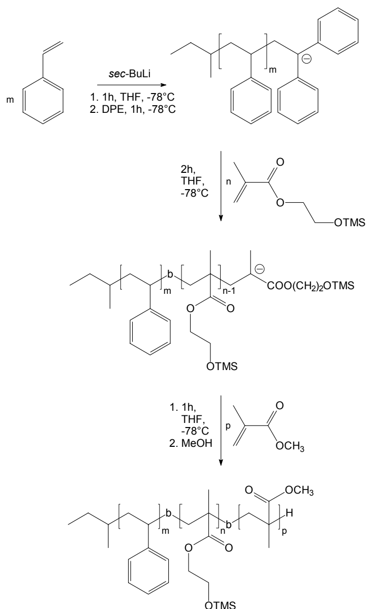
Scheme 3-1: Synthesis of PS- b -PHEMA- b -PMMA (SHM) triblock copolymers.
