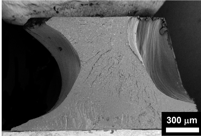
Figure 5-4: Cross sectional SEM image of a protrusion formed during exposure to a DC electric field (1.8 kV/mm).
