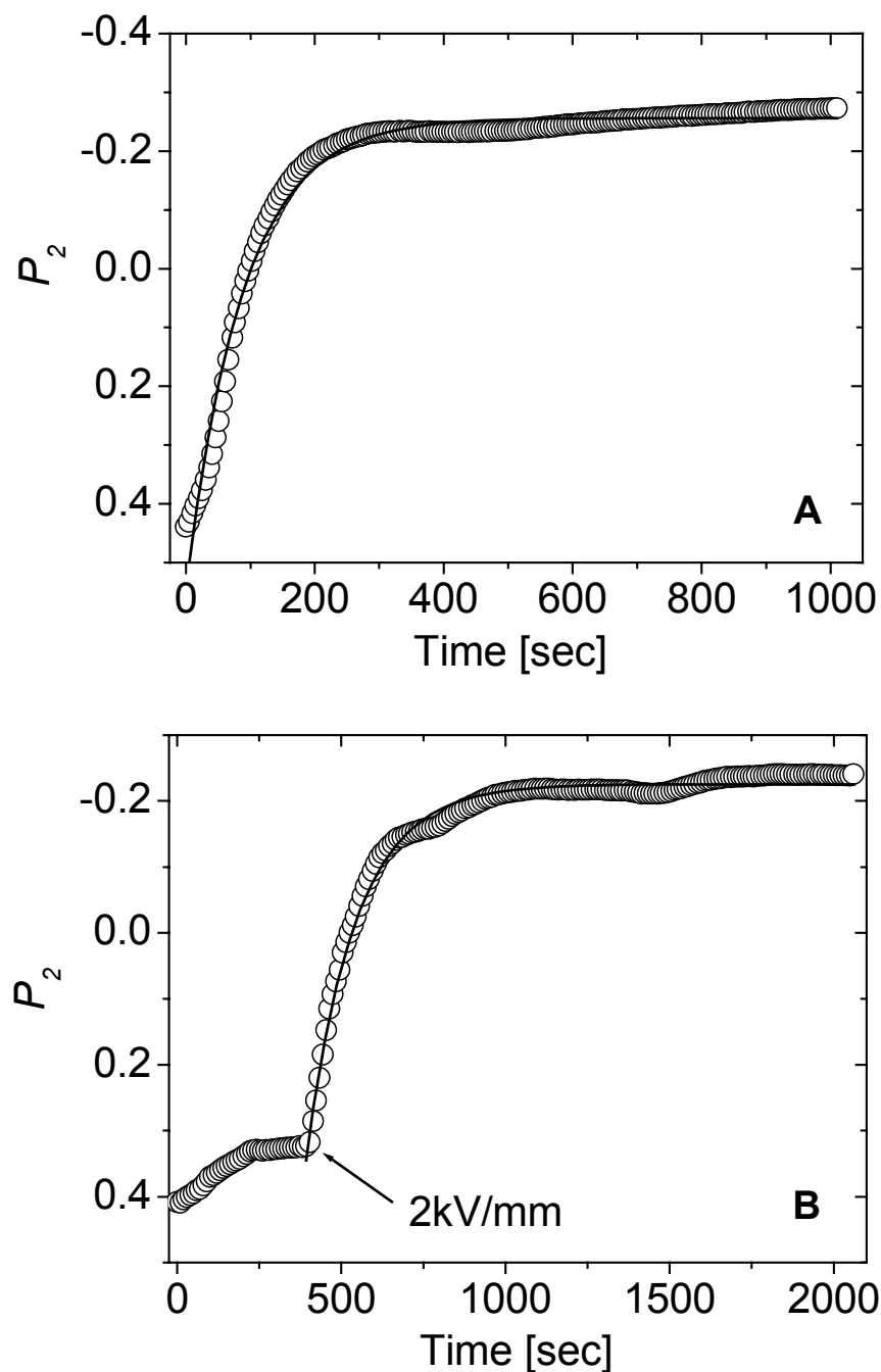
Figure 7-5: Evolution of orientational order parameter P_2 with time (for orientation parallel to the electric field vector): (A) 40 wt.-% solution of S_{47}H_{10}M_{43}^{82} in THF at 1 kV/mm, (B) 45 wt.-% solution of S_{47}H_{10}M_{43}^{82} in THF at 1 kV/mm and 2 kV/mm. The solid lines represent least squares fits to the data according to Equation 6-3.
