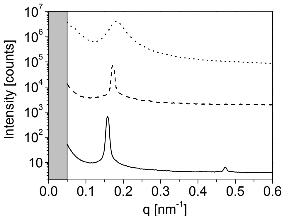
Figure 7-1: Scattering intensity profiles of S_{47}H_{10}M_{43}^{82} solutions in THF at various concentrations. 37.5 wt.-% (.....), 40 wt.-% (---), 47.5 wt.-% (—).
