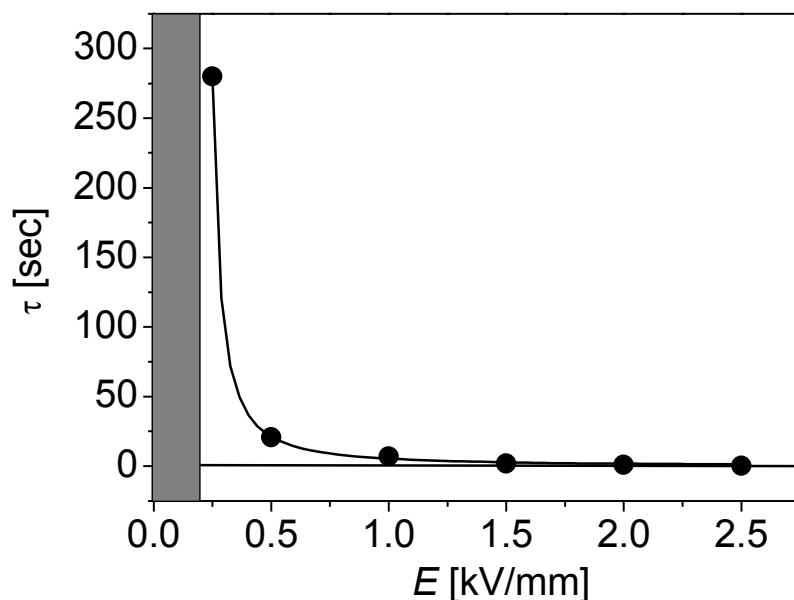
Figure 8-7: Electric Field dependence of time constant \tau for 40 wt.-% solutions of a S_{50}V_{50}^{78} diblock copolymer in THF. Electrode distance: 2mm. The solid line represents a least squares fit of the power law \tau = \alpha(E - E_t)^a + \tau_\infty to the data yielding \alpha = 0.19 sec, a = -1.4 , E_t = 200 V/mm, and \tau_\infty = 0 sec.
