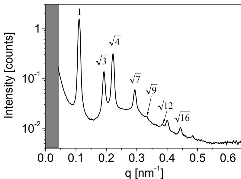
Figure 8-11: Scattering intensity profile of a 40 wt.-% solution of S_{16}V_{21}T_{63} 138 in THF.
