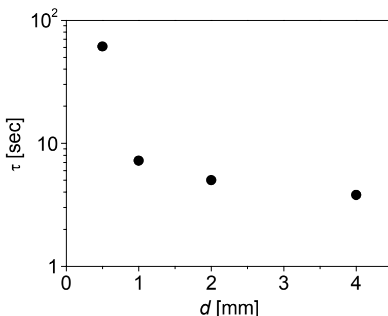
Figure 6-18: Logarithmic dependence of the orientation kinetics on the electrode spacing for a 35 wt.-% solution of SI-80 in toluene at 1 kV/mm.
