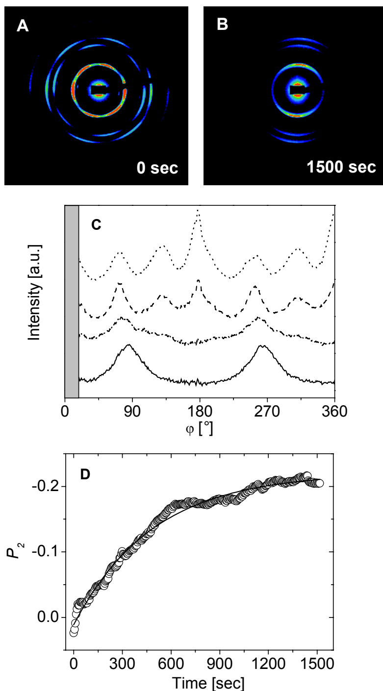
Figure 8-12: 2D SAXS pattern of a 40 wt.-% solution of S_{16}V_{21}T_{63}^{138} in THF (A) prior to and (B) after application of the electric field. (C) Azimuthal angular dependence of the scattering intensity for a 40 wt.-% solution of S_{16}V_{21}T_{63}^{138} in THF at 2 kV/2 mm: 0 sec (.....), 45 sec (---), 330 sec (-.-), 1500 sec (—). (D) Time evolution of orientational order parameter P_2 for the same system: \tau = 480 sec, P_{2,\infty} = -0.23 .
