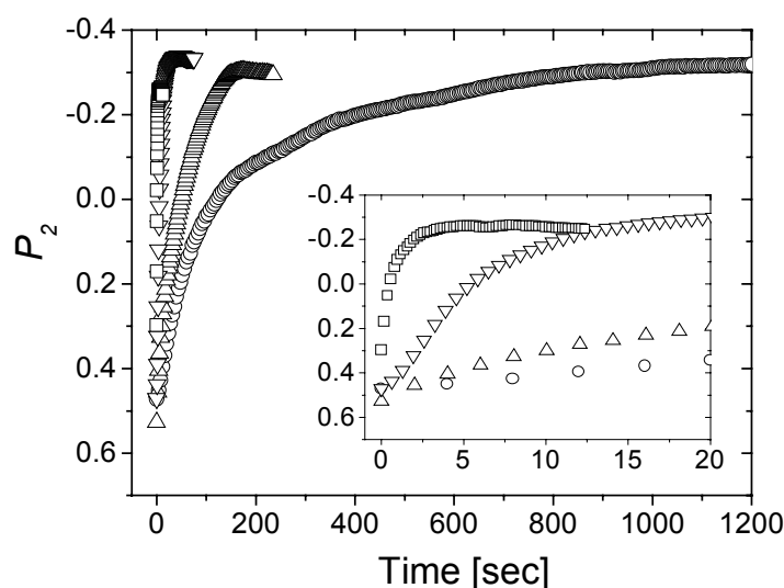
Figure 6-6: Evolution of orientational order parameter P_2 with time for different concentrations at 2 kV/2 mm ( \square = 34.5 wt.-%, \nabla = 37.5 wt.-%, \triangle = 42.5 wt.-%, \circ = 50 wt.-%).
