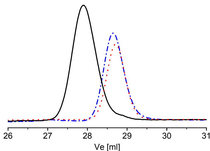
Figure 3-1: GPC trace (RI signal) of triblock copolymer S_{47}H_{10}M_{43} 82 (—) and its precursors PS (.....) and PS- b -PHEMA (-.-.). M_n = 82300 g/mol, M_w/M_n = 1.04
