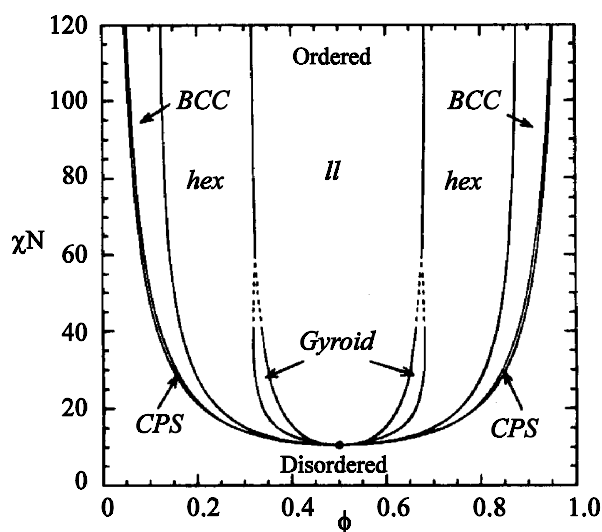
Figure 1-4: Phase diagram for diblock copolymers in the strong segregation limit (SSL) as calculated by Matsen et al. 16
