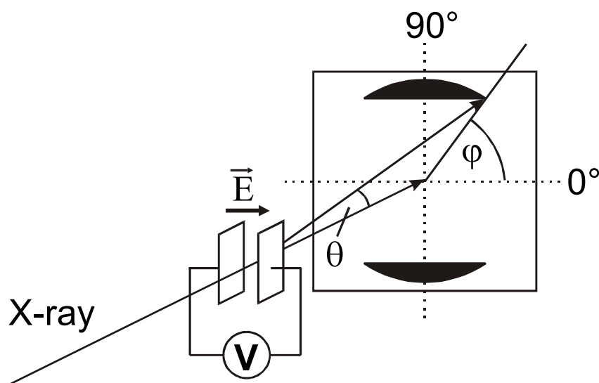
Figure 6-1: Experimental setup for in-situ SAXS.
