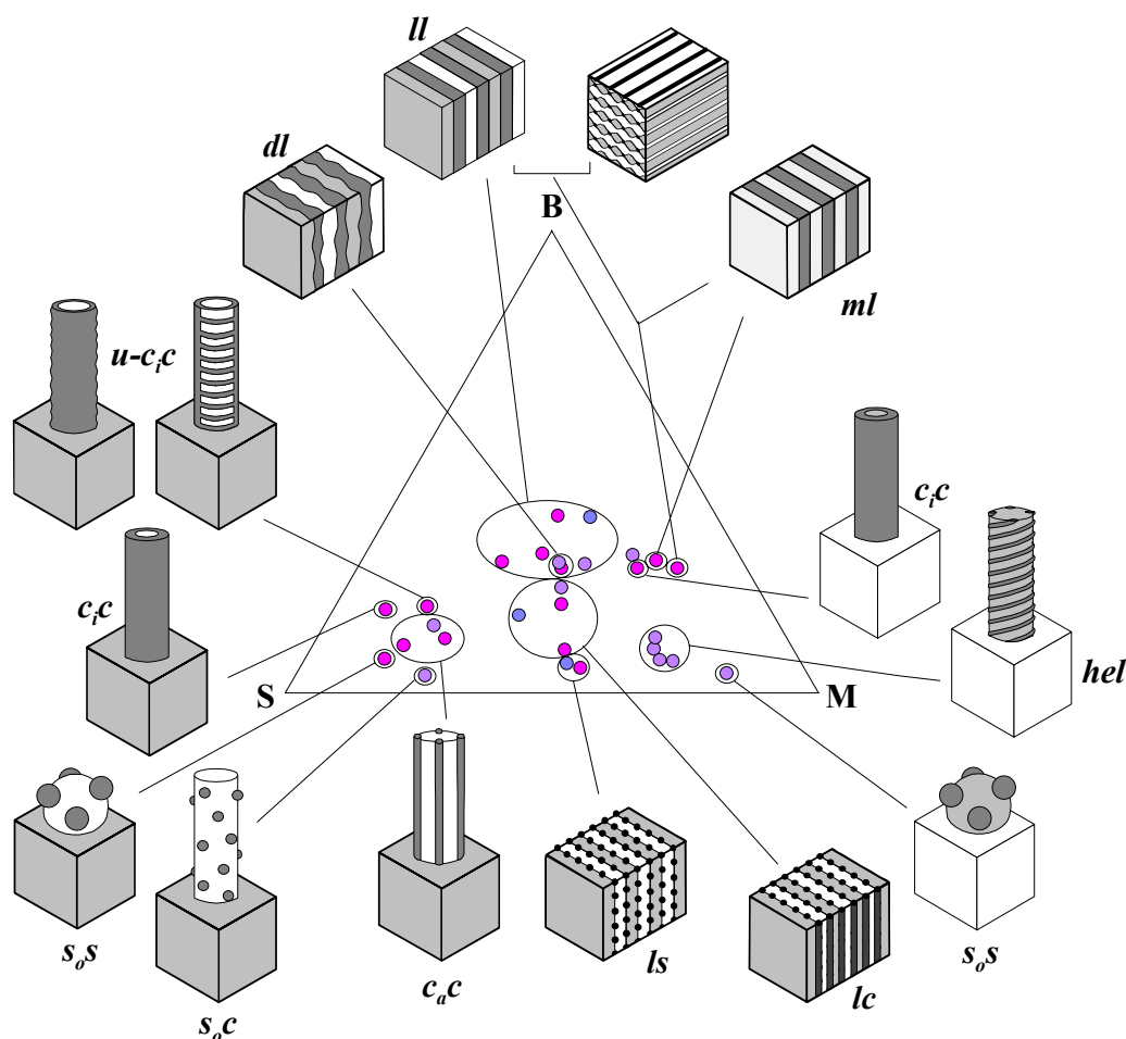
Figure 1-6: Ternary phase diagram of SBM triblock copolymers, color according to staining with \text{OsO}_4 . PS: grey, PB: black, PMMA: white.
