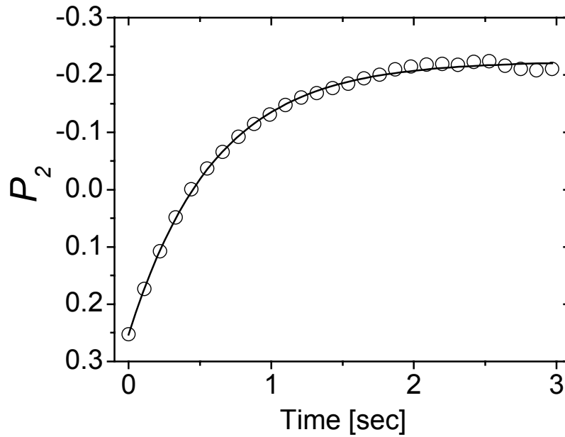
Figure 8-5: Evolution of the orientational order parameter P_2 for a 40 wt.-% solution of a S_{50}V_{50}^{78} diblock copolymer in THF ( E = 4 \text{ kV/2 mm} ). The solid line is a least squares fit to the data according to Equation 6-3 with P_{2,0} = 0.26 , P_{2,\infty} = -0.22 , and \tau = 0.86 \text{ sec} .
