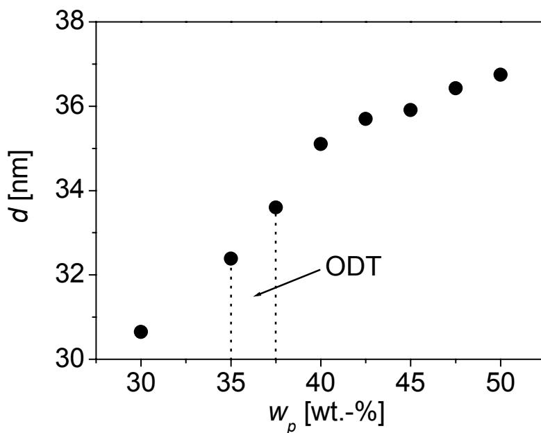
Figure 8-2: Concentration dependence of the lamellar spacing for S_{50}V_{50} 78 solutions in THF ( d_{bulk} = 43 nm).
