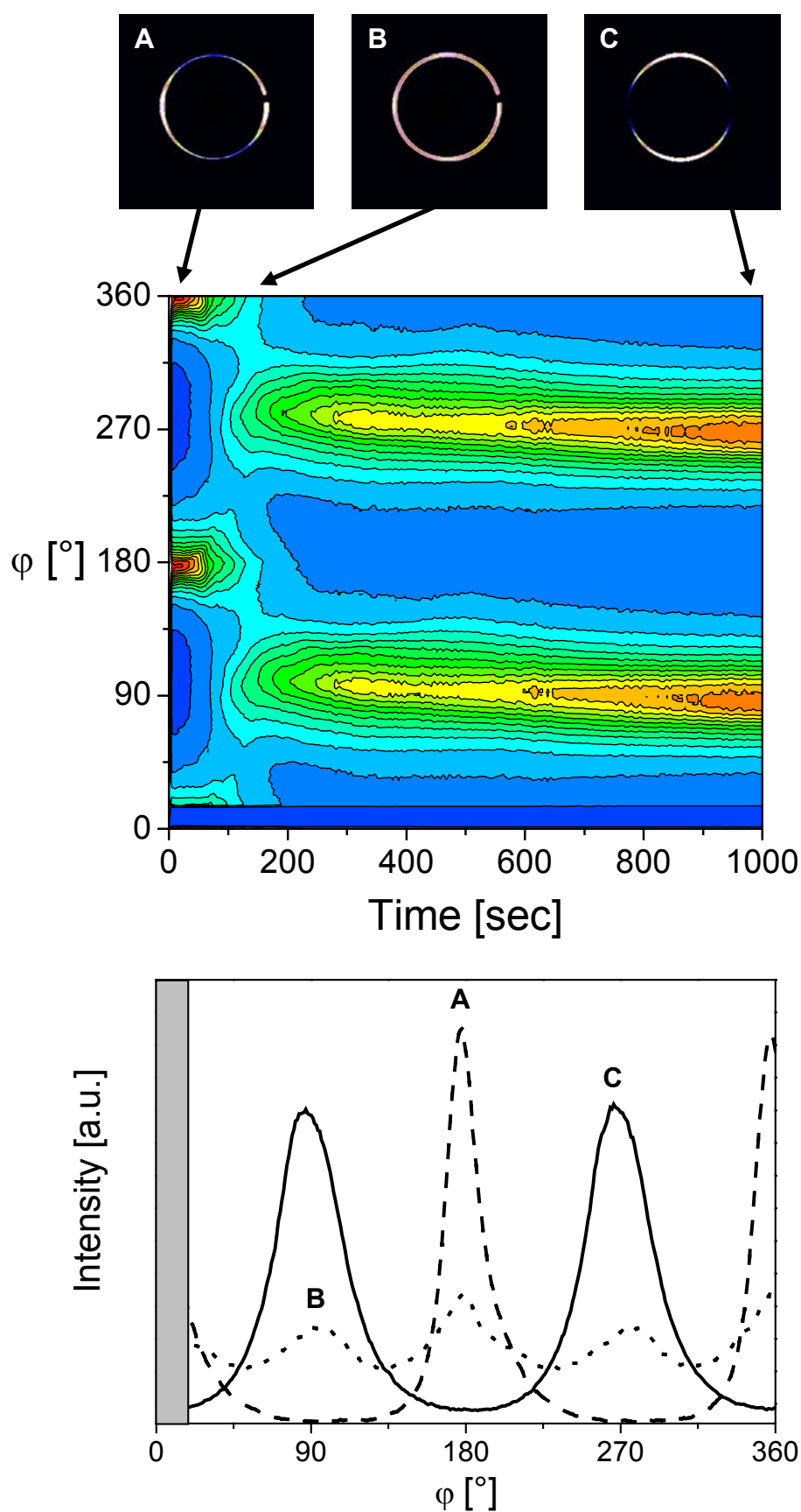
Figure 7-4: Scattering profiles and azimuthal angular dependence of the scattering intensity of a 40 wt.-% solution of S_{47}H_{10}M_{43}^{82} in THF at 1 kV/mm; (A) t = 0 sec, (B) t = 100 sec, (C) t = 985 sec
