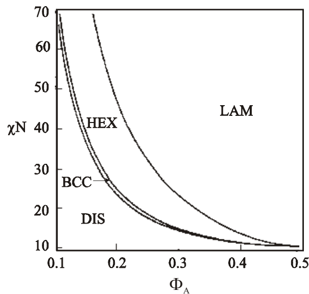
Figure 1-2: Phase diagram for diblock copolymers in the weak segregation (WSL) limit calculated by Leibler 14
