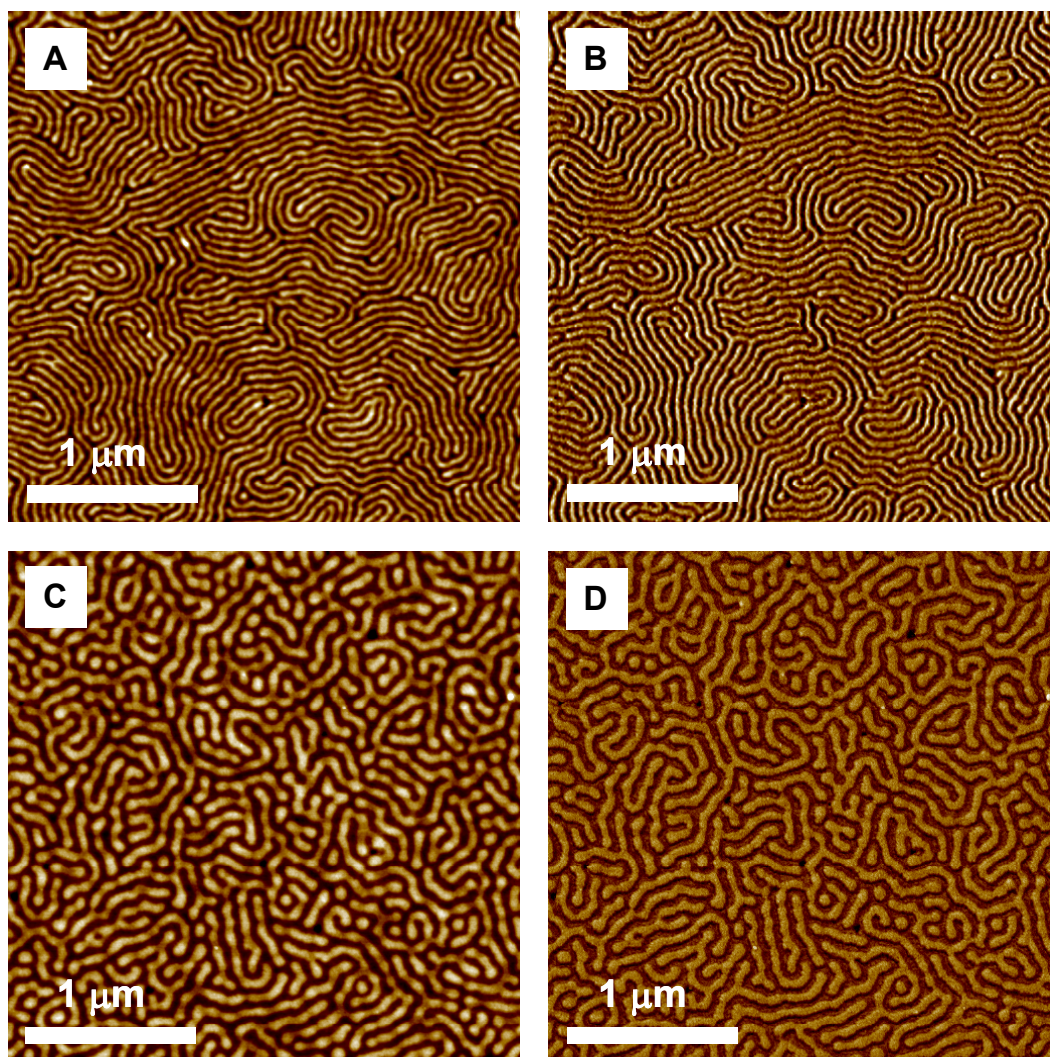
Figure 3-2: SFM topography (a,c) and phase images (b,d) of thin films dip-coated from 1 mg/ml THF solutions onto a polished silicon wafer: (a, b) 15 nm thick film of S_{46}H_4M_{50} 134 ; (c, d) 25 nm thick film of S_{56}2VP_6M_{38} 299 . Topography: 8 nm, Phase: 8 °.
