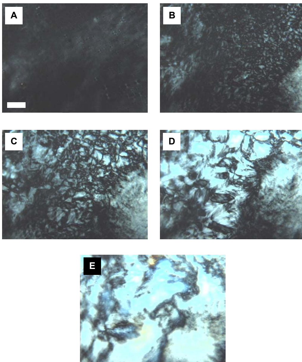
Figure 6-17: Polarizing optical micrographs of a 40 wt.-% solution of SI-80 in toluene between two ITO covered glass slides ( d = 2\text{mm} ) at 4 kV. (A) prior to electric field, (B) after 1 min, (C) 2 min, (D) 3 min and (E) 5 min. The viewing direction is parallel to the electric field vector. The scale bar represents 200 \mu\text{m} .
