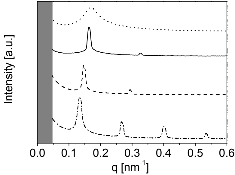
Figure 6-2: Scattering intensity profiles at various concentrations. 34 wt.-% (.....), 35 wt.-% (—), 50 wt.-% (---), 70 wt.-% (-.-).
