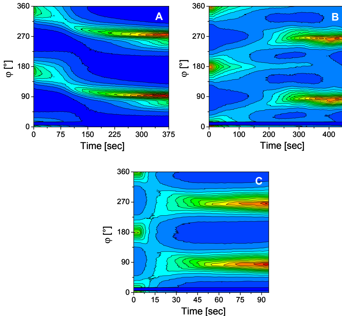
Figure 6-11: Azimuthal angular dependence of the scattering intensity for different temperatures at 2 kV/2 mm. (A) 27.3°C, (B) 51.5°C, (C) 80°C.
