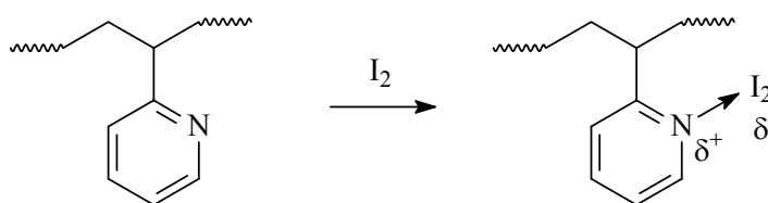
Figure 2-7: Formation of a charge-transfer complex between iodine and 2-vinyl pyridine.
