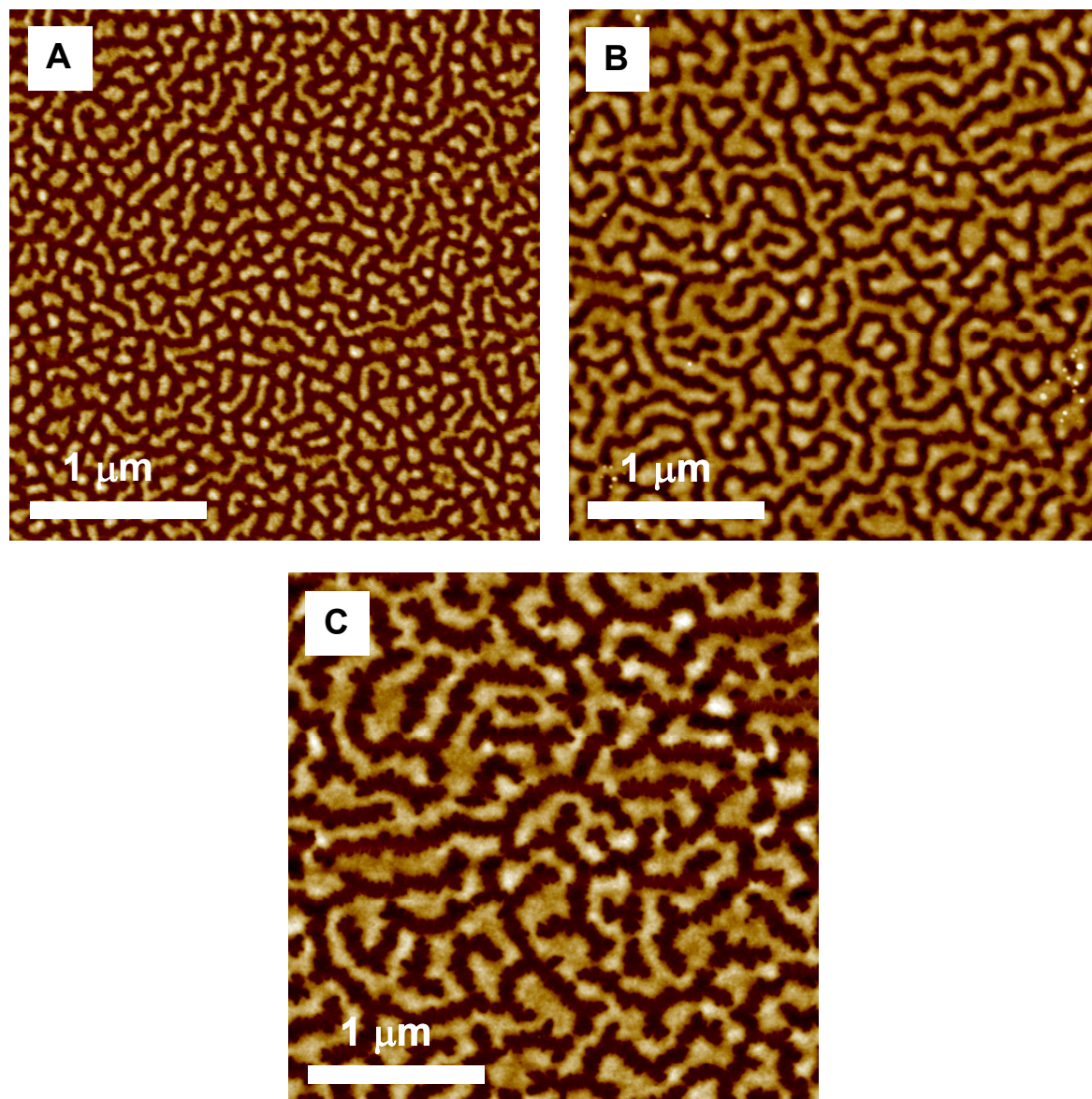
Figure 3-4: SFM micrographs of ultrathin films of PS- b -P2VP- b -PMMA adsorbed from 1 mg/ml THF solutions onto a polished silicon wafer. (a) S_{51} 2VP_5 M_{44}^{110} ; (b) S_{48} 2VP_5 M_{47}^{180} ; (c) S_{56} 2VP_6 M_{38}^{299} . Z-range: 8 nm.
