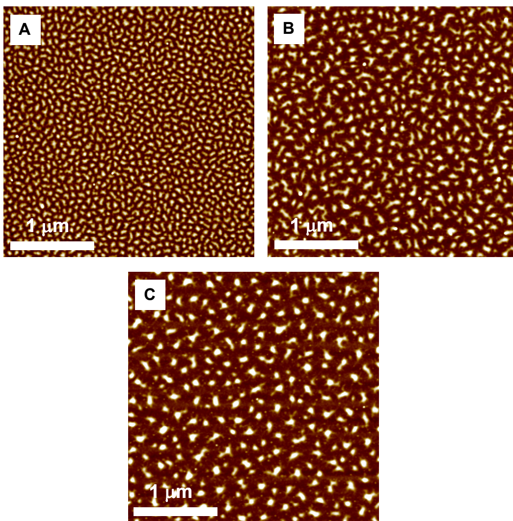
Figure 3-6: SFM micrographs of ultrathin films adsorbed from 1 mg/ml THF solutions onto a polished silicon wafer after annealing for 8 days at 170 °C in vacuum. (a) S_{47}H_{10}M_{43}^{82} (Z-range: 6 nm); (b) S_{67}H_6M_{27}^{129} ; (c) S_{56}2VP_6M_{38}^{299} , Z-range: 10 nm (b/c).
