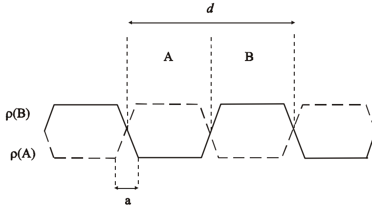
Figure 1-3: Characteristic composition profile in the case of strong segregation limits (SSL) 11
