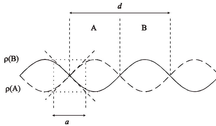
Figure 1-1: Sinusoidal composition profile for phase-separated AB diblock copolymers in the weak segregation limit (WSL) 11
