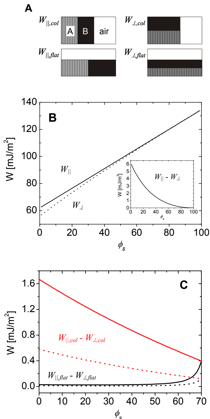
Figure 7-10: (A) Four basic geometries of lamellar orientation. Calculated differences in energy stored in the capacitor between lamellar alignment parallel and perpendicular to the electric field vector in dependence of solvent volume fraction; (B) SHM solution in THF in closed capacitor; (C) open capacitor which allows for solvent evaporation with SHM (—) and with SM block copolymer (....) in CHCl 3 .
