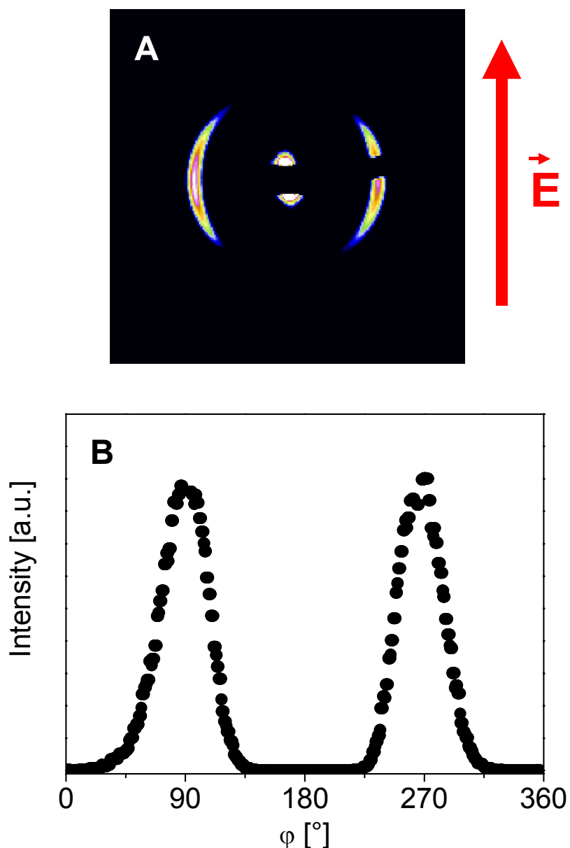
Figure 7-9: SAXS data of a SHM bulk sample prepared from a 40 wt.-% solution dried under an applied electric field of 1 kV/mm. (A) 2D-SAXS pattern and (B) azimuthal intensity distribution at first-order reflection ( P_2 = -0.4 ). 1
