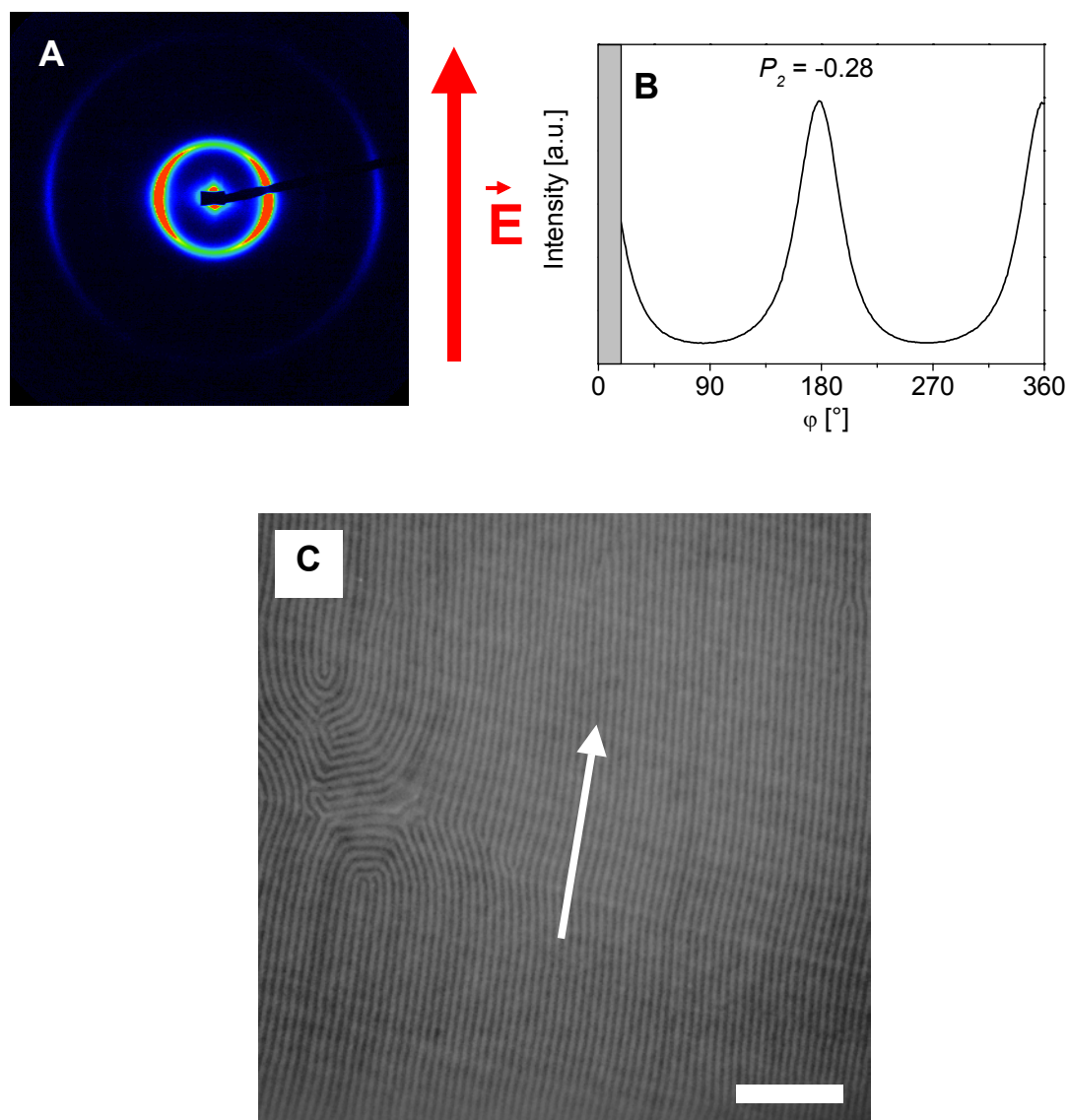
Figure 8-6: SAXS and TEM data of a S_{50}V_{50}^{78} melt sample prepared from a 37.5 wt.-% solution cast in the presence of an electric field of 2 kV/mm. (A) 2D-SAXS pattern and (B) azimuthal intensity distribution at first order reflection. (C) TEM micrograph (stained with iodine). The arrow indicates the direction of the electric field vector. The scale bar represents 500 nm.
