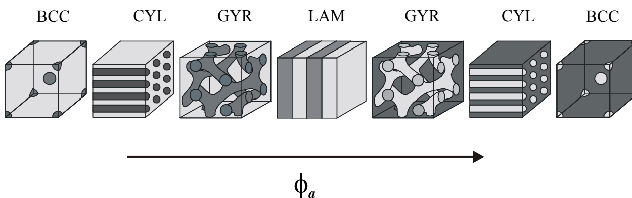
Figure 1-5: Thermodynamic equilibrium morphologies in AB diblock copolymers depending on the volume fraction of component A.
