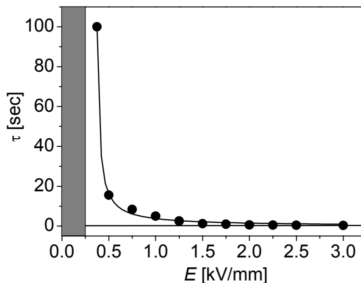
Figure 6-10: Electric field dependence of time constant for 35 wt.-% solutions (electrode spacing: 2 mm). The solid line represents a least-squares fit to the power law \tau = \alpha(E - E_0)^a + \tau_\infty to the data points.
