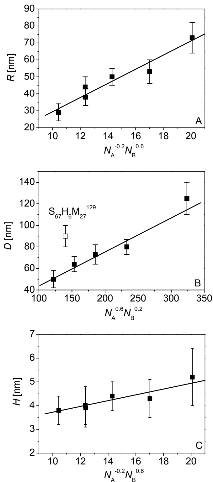
Figure 3-9: Scaling of PS- b -PHEMA- b -PMMA and PS- b -P2VP- b -PMMA stripe morphology. (A) half-width R , (B) half-distance D , (C) height H of PS stripes.
