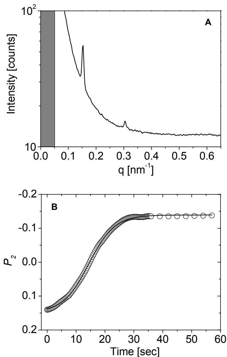
Figure 8-8: (A) Scattering intensity profile of a 50 wt.-% solution of S_{50}T_{50}^{100} in THF. (B) Evolution of orientational order parameter with time for a 40 wt.-% solution of S_{50}T_{50}^{100} in THF at 2 kV/mm: \tau = 9.7 sec, P_{2,\infty} = -0.14 .
