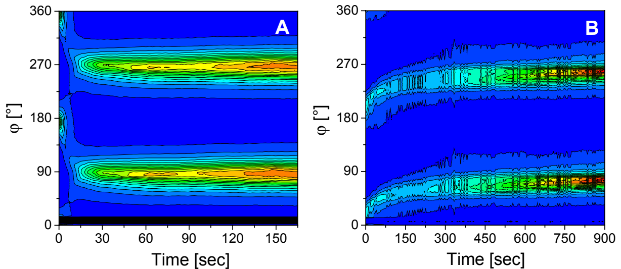
Figure 6-8: Azimuthal angular dependence of the scattering intensity for different concentrations at 2 kV/2 mm. (A) 35 wt.-%, (B) 50 wt.-%.
