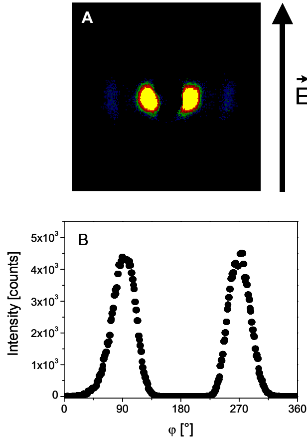
Figure 5-5: (A) 2D-SAXS pattern of a film cast in the presence of a DC electric field (1.8 kV/mm). The experiment has been performed within one of the columns bridging between the electrodes. The lamellae are oriented preferentially along the field direction. (B) azimuthal intensity distribution at first order reflection ( P_2 = -0.4 ).
