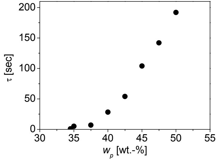
Figure 6-7: Concentration dependence of time constant \tau .
