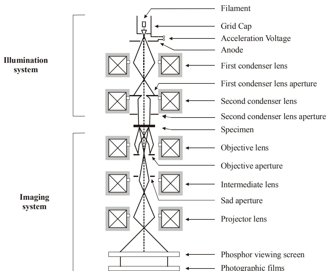
Figure 2-4: Schematic cross section of a transmission electron microscope 37
