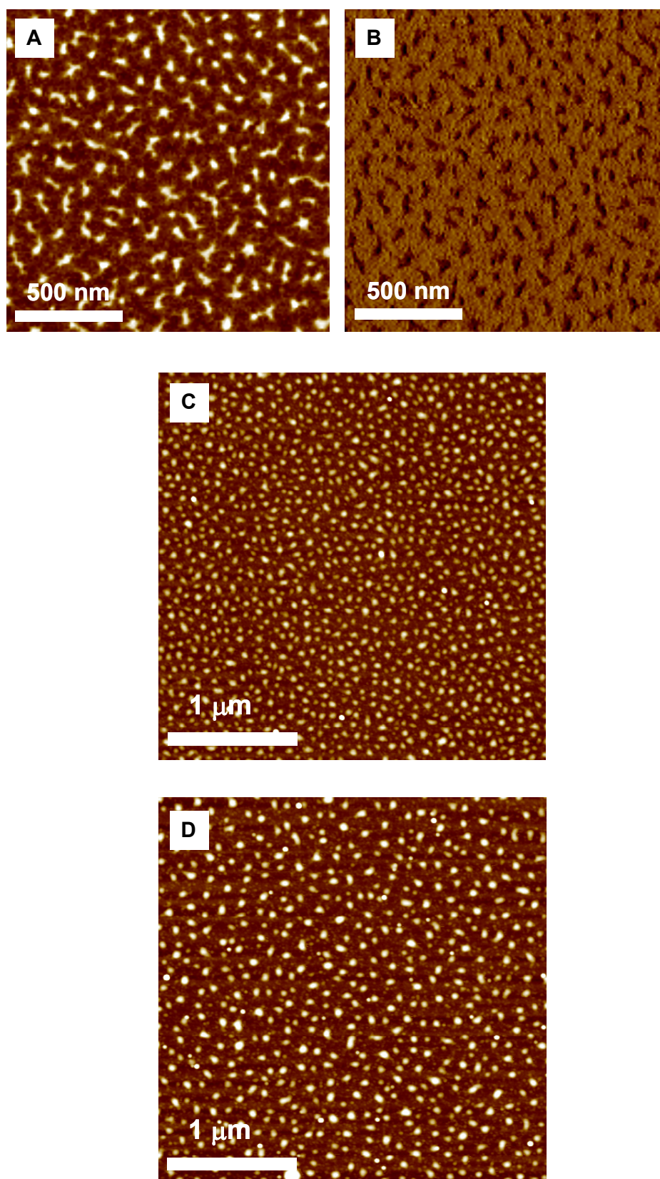
Figure 3-8: SFM micrographs of ultrathin films dip-coated from 0.01 mg/ml THF solutions onto a polished silicon wafer: S_{46}H_4M_{50}^{134} (a) topography (5 nm) and (b) phase (15 degrees) as-prepared and (c) after annealing for 5 days at 190 °C; (d) S_{48}2VP_5M_{47}^{180} after annealing for 5 days at 190 °C. Z-range: 10 nm (c/d).
