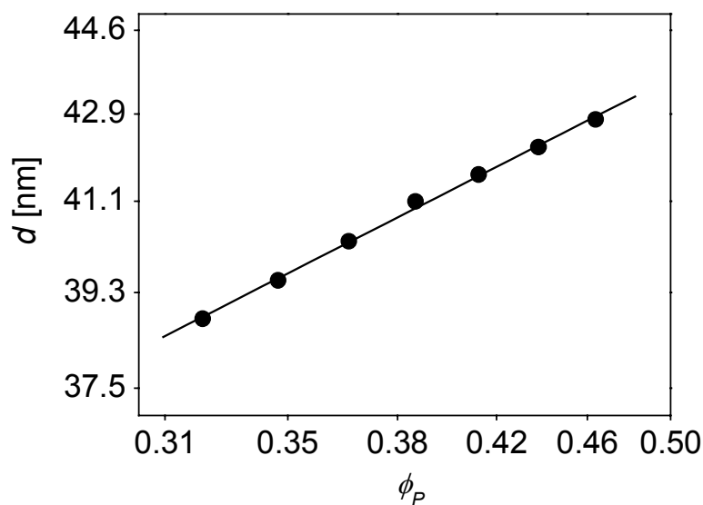
Figure 6-4: Double logarithmic plot of dependence of lamellar spacing on the volume fraction of polymer \phi_P ( d \sim \phi_P^{0.30 \pm 0.01} ).
