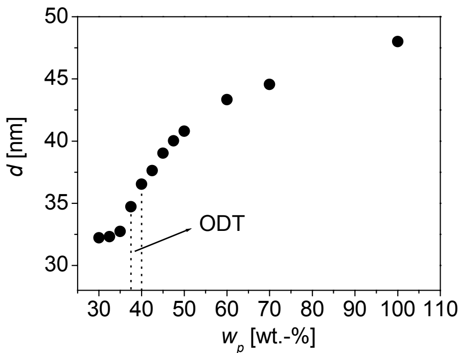
Figure 7-2: Concentration dependence of the lamellar spacing ( d_{100} ).
