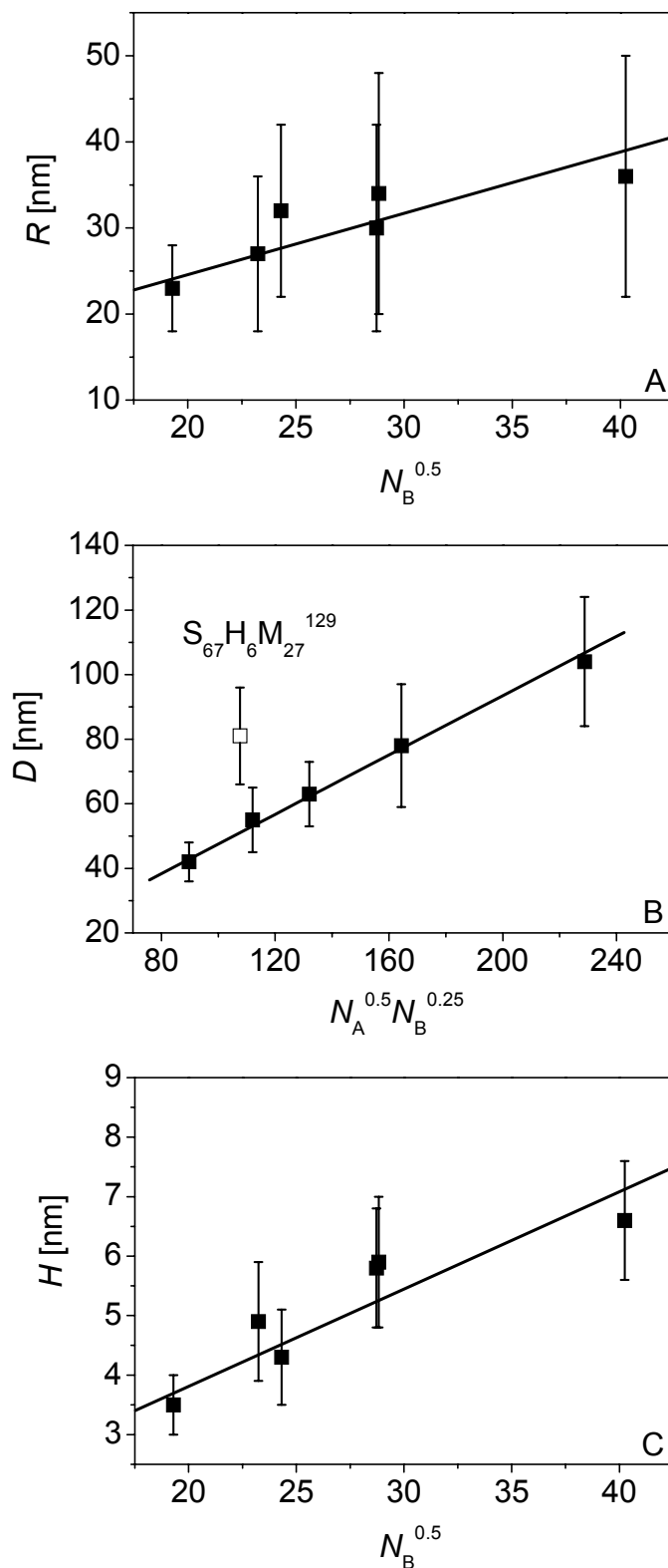
Figure 3-10: Scaling of PS- b -PHEMA- b -PMMA and PS- b -P2VP- b -PMMA island morphology. (A) half-width R , (B) half-distance D , (C) height H of PS islands.
