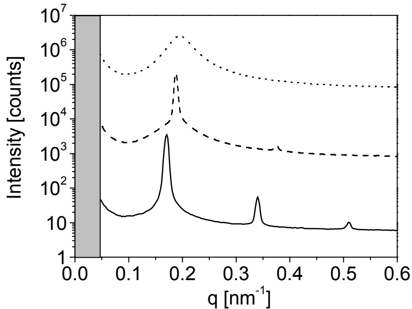
Figure 8-1: Scattering intensity profiles of S_{50}V_{50}^{78} solutions in THF at various concentrations. 35 wt.-% (.....), 37.5 wt.-% (---), 50 wt.-% (—).
