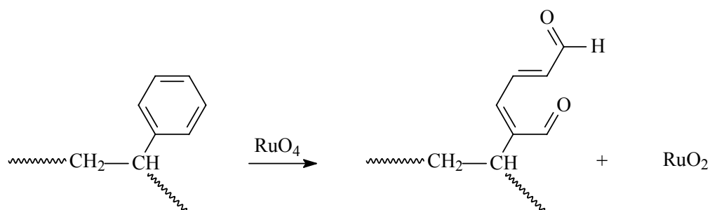
Figure 2-5: Reaction of \text{RuO}_4 with aromatic double bonds
