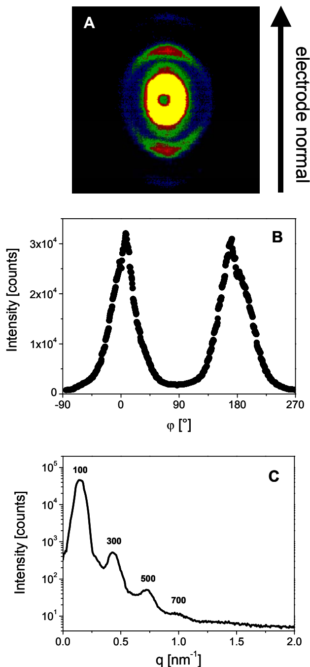
Figure 5-2: (A) 2D-SAXS pattern of a film cast under zero-field conditions. The lamellae are aligned parallel to the boundary surfaces (electrodes). (B) azimuthal intensity distribution at q^* = 0.14 \text{ nm}^{-1} (corresponding to first order reflection). (C) azimuthally integrated intensity as a function of scattering vector q .
