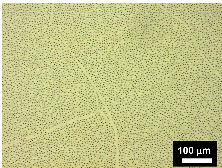
Figure 4-6: Optical micrograph of PS 14 on S_{48}VP_5M_{47}^{180} after CHCl_3 vapor treatment for 5.5 min.
