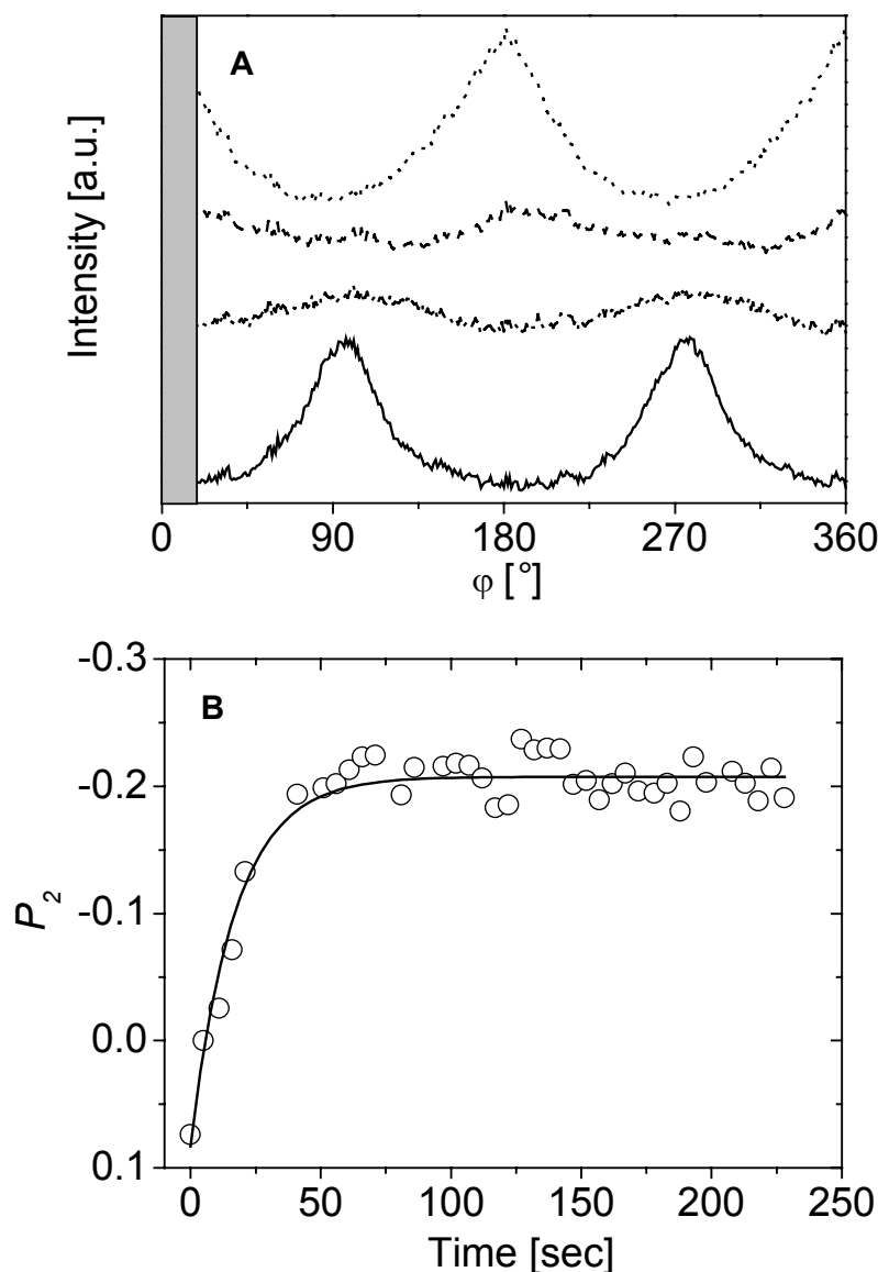
Figure 8-10: (A) Azimuthal angular dependence of the scattering intensity for a 40 wt.-% solution of S_{27}V_{35}T_{38}^{84} in THF at 2 kV/2 mm: 0 sec (.....), 5 sec (---), 10 sec (-.-), 85 sec (—). (B) Time evolution of P_2 for the same system, \tau = 17.7 sec, P_{2,\infty} = -0.21 .
