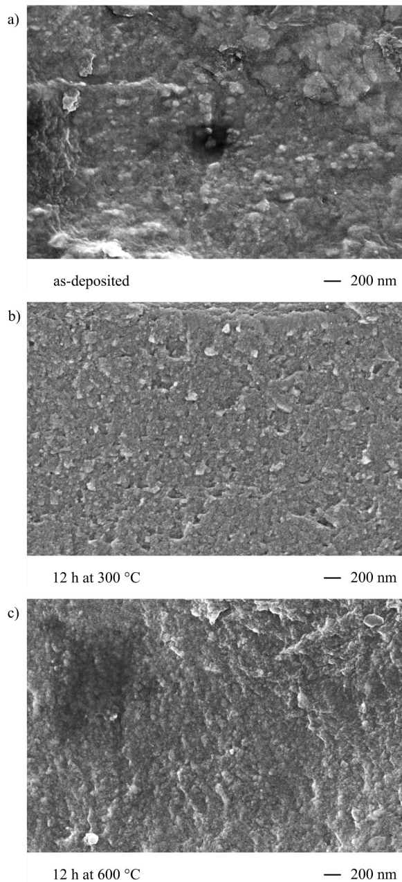
Fig. 9. SEM fracture images of TiO 2 PAD films in the as-deposited state (a), after heat treatment at 300 °C (b) and 600 °C (c).
