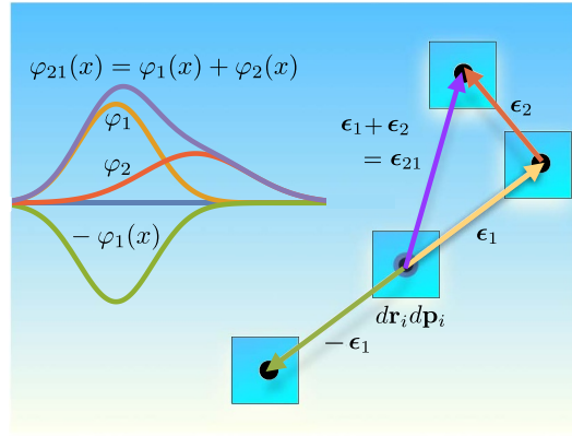
Figure 1. Group structure of the gauge transformations in electrodynamics (curves) and in statistical mechanics (arrows), depicted for global transforms for the latter case. Shown are different forms of the scalar gauge function \varphi(x) that parameterizes the transform in electrodynamics. A given gauge function \varphi_1(x) has an inverse -\varphi_1(x) . Two transforms \varphi_1(x) and \varphi_2(x) combine additively to \varphi_{21}(x) = \varphi_1(x) + \varphi_2(x) . For the statistical mechanics the global gauge invariance is shown for different realizations of a constant shifting vector \epsilon_1 . The inverse transform \epsilon_{-1} = -\epsilon_1 . Two transformations that correspond to \epsilon_1 and \epsilon_2 combine additively to \epsilon_{21} = \epsilon_1 + \epsilon_2 . Also illustrated is the conserved phase space volume element dx_i dp_i .
