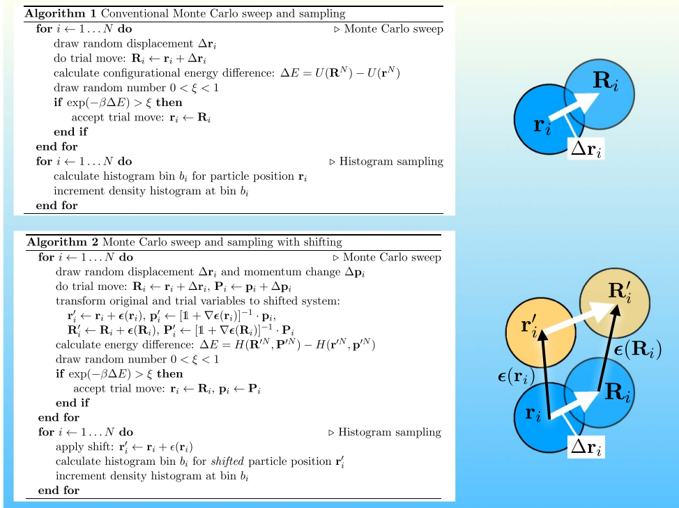
Figure 7. Pseudocodes that describe Monte Carlo simulations in the standard form (algorithm 1) and using phase space shifting (algorithm 2). The standard Metropolis algorithm is based on trial displacement from \mathbf{r}_i, \mathbf{p}_i to \mathbf{R}_i, \mathbf{P}_i , where the capitalization indicates the trial variables. In the shifted system the transformation is applied both to the current state, resulting in \mathbf{r}'_i, \mathbf{p}'_i , as well as to the trial state, resulting in \mathbf{R}'_i, \mathbf{P}'_i . The Metropolis criterion is then evaluated with respect to the shifted variables and these then also form the basis for the sampling of observables. The illustrations of the shifted system only display configurational degrees of freedom with the momentum variables being treated accordingly. The pseudocode for histogram sampling in the shifted system only describes the configurational strategy with corresponding momentum sampling being required for obtaining, e.g. the one-body phase space distribution function f(\mathbf{r}, \mathbf{p}) shown in figure 6.
