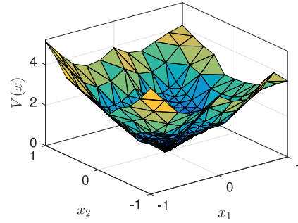
Fig. 2. Piecewise affine PCLF for Artstein's circles.
