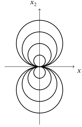
Fig. 1. Invariant sets for the solutions of (14).
