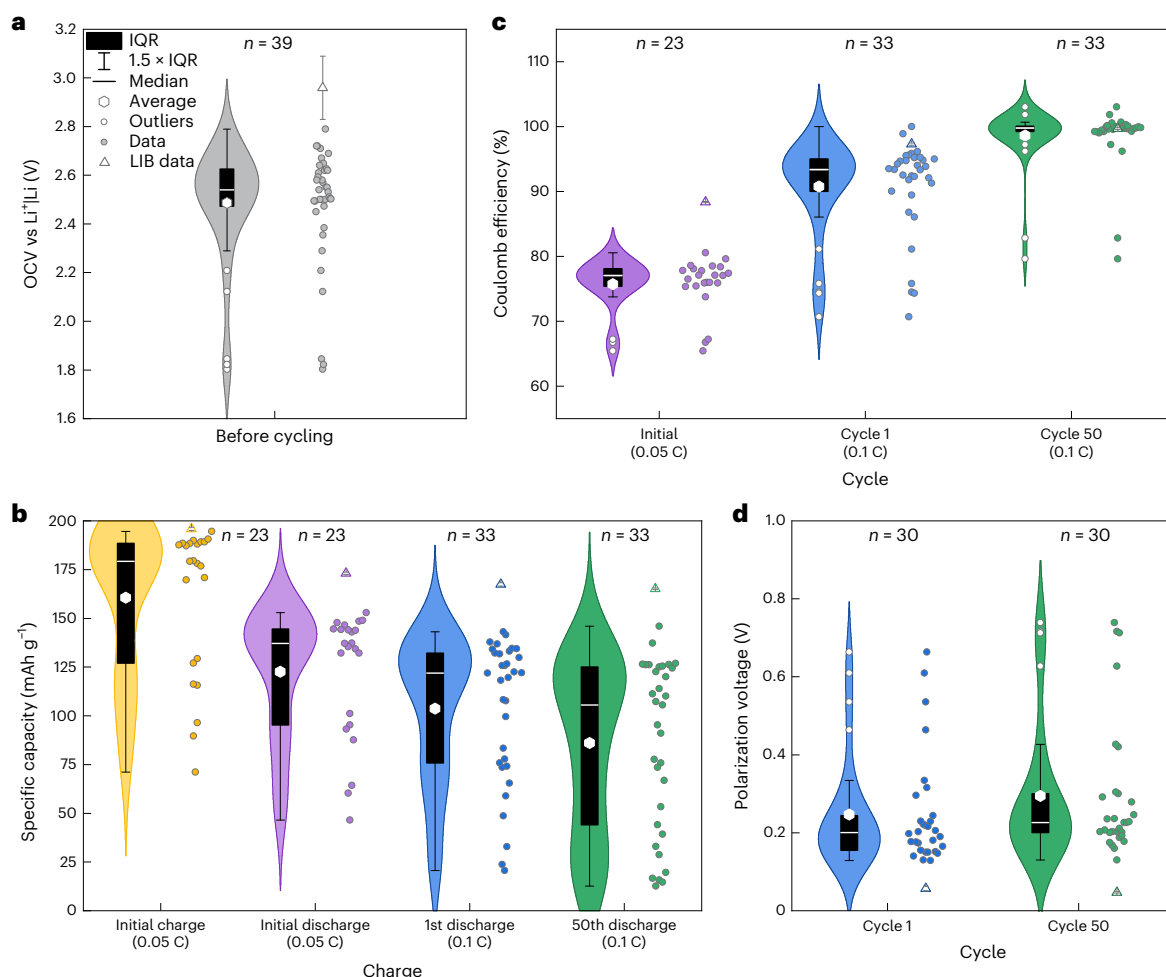
Fig. 2 | Analysis of various cell performance figures of merit. a–d , Violin plots showing the open circuit voltage (OCV) of all cells, measured after assembly, and converted to vs. \text{Li}^+/\text{Li} ( a ); specific (dis-)charge capacities of the pretreatment and 0.1 C cycling ( b ); Coulomb efficiencies ( c ) and polarization voltage ( d ), calculated from average charge minus average discharge voltage of the respective cycle. Boxes inside the violin diagrams show the IQR, whiskers extend
