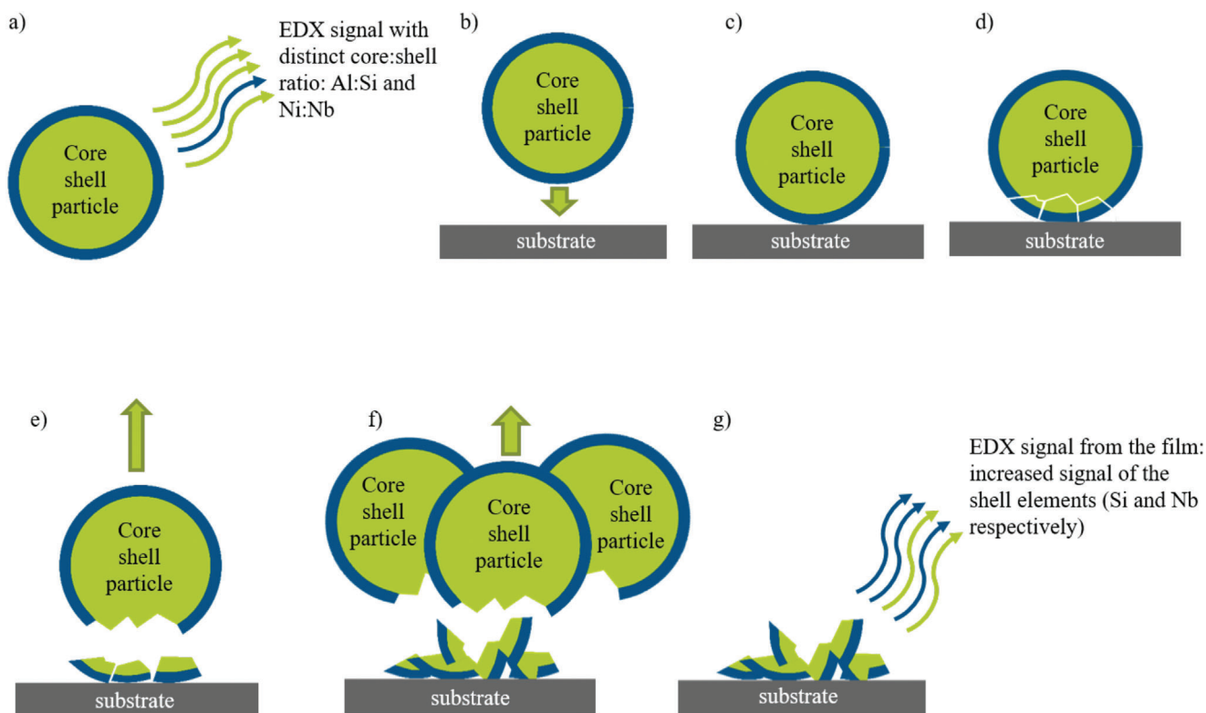
Figure 13. Initially, the element ratio between core and shell is determined by EDX before spraying (a). The particles are accelerated by the gas flow toward the substrate (b) and impact at the substrate (c). The particle fragment (d) and a part of the shell as well as a part of the core is deposited. Subsequent particles undergo the same process and form the film. The final film is characterized by EDX (g) whereas a significantly more deposited shell material can be determined.
