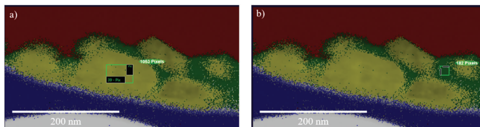
Figure 10. STEM–EDX image at \text{Al}_2\text{O}_3:\text{SiO}_2 films with a color-indicating element composition. Two areas are analyzed respectively. a) The evaluation area of the aluminum-rich area and b) the silicon-rich area.
