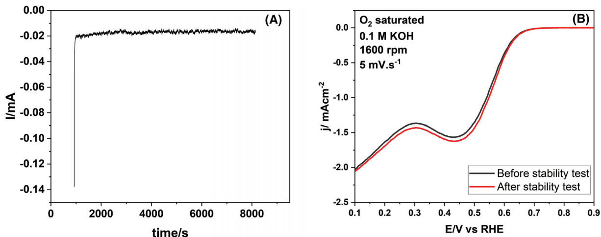
FIGURE 10 (A) Stability test (chrono-amperometric [CA]) of TiN@Si-Al-C-N 1000 performed in O 2 -saturated 0.1 M KOH at 0.6 V for 2 h. (B) cyclic voltammograms (CVs) (anodic scan) of TiN@Si-Al-C-N 1000 , performed in O 2 -saturated 0.1 M KOH solution with a slow scan rate of 5 mV/s (1600 rotation)
