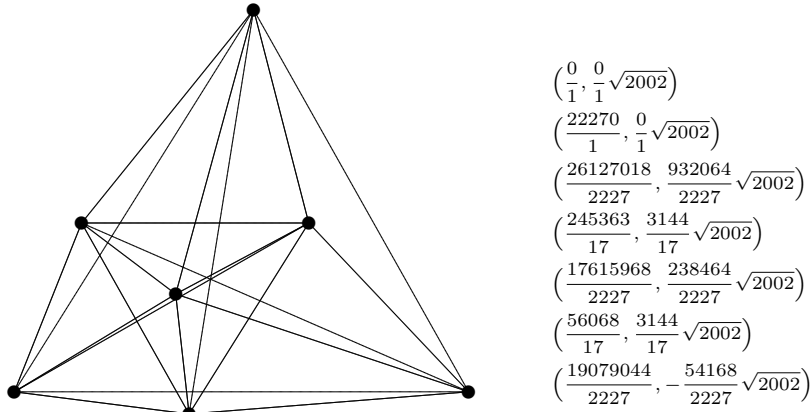
Figure 1: First example of an integral heptagon in general position.
