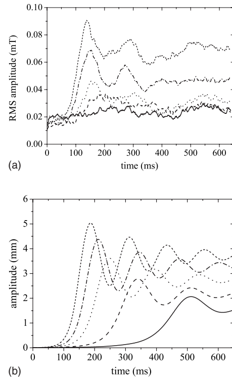
FIG. 5. Time-resolved amplitudes for the fluid EMG 909. (a) Measurements for increasing supercritical inductions \hat{B} = 0.028 (full line), 0.057 (dashed line), 0.100 (dotted line), 0.157 (dash-dotted line), and 0.200 (short-dashed line). For clearer appearance, the plotted lines are smoothed by averaging ten neighboring points of the original data set. (b) Numerical results for \hat{B} = 0.028 (full line), 0.058 (dashed line), 0.103 (dotted line), 0.153 (dashed-dotted line), and 0.203 (short-dashed line).
