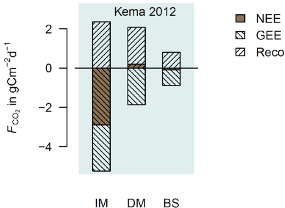
Figure 5. Simulated carbon fluxes at Kema in 2012 (46 days: 12 July to 26 August 2012) for IM, DM, and BS. Hatched bars denote the simulated GEE and R_{eco} , the sum is the NEE (brown bar).
