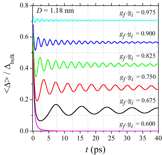
Figure 4. The time evolution of the spatially averaged order parameter \overline{\Delta}(t) after a sudden perturbation with different strengths, characterized by a different ratio between final and initial value of the coupling strength. g_i is kept fixed to the value for lead.
