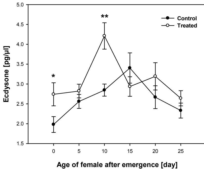
Fig. 20. Ecdysone titer in the haemolymph of B. dubia females treated with methoprene (100 \mu\text{g}/\text{female} ) (open circles) or with 5 \mu\text{l} acetone (control, closed circles) during the period of ovarian growth. Data are expressed as means \pm S.E. (* p < 0.05 ; ** p < 0.01 ) indicate significant differences between control and methoprene treated females (t-test d 0, 5, 15, 25; Mann-Whitney Rank Sum Test d 10, 20); n = 10 .
