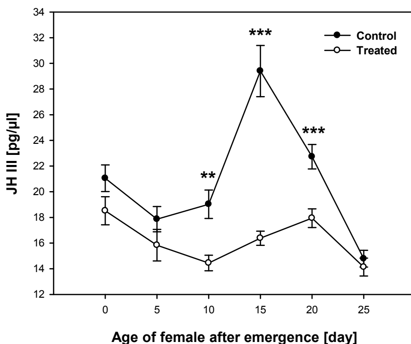
Fig. 29. JH III titer in the haemolymph of B. dubia females, treated with pyriproxyfen (100 \mu\text{g}/\text{female} ) (open circles) or with 5 \mu\text{l} acetone (control, closed circles) during the period of ovarian growth. Data are expressed as means \pm S.E. (** p < 0.01 ; *** p < 0.001 ) indicate significant differences between control and pyriproxyfen treated females (t-test; Mann-Whitney Rank Sum Test d 0, 15); n = 10 .
